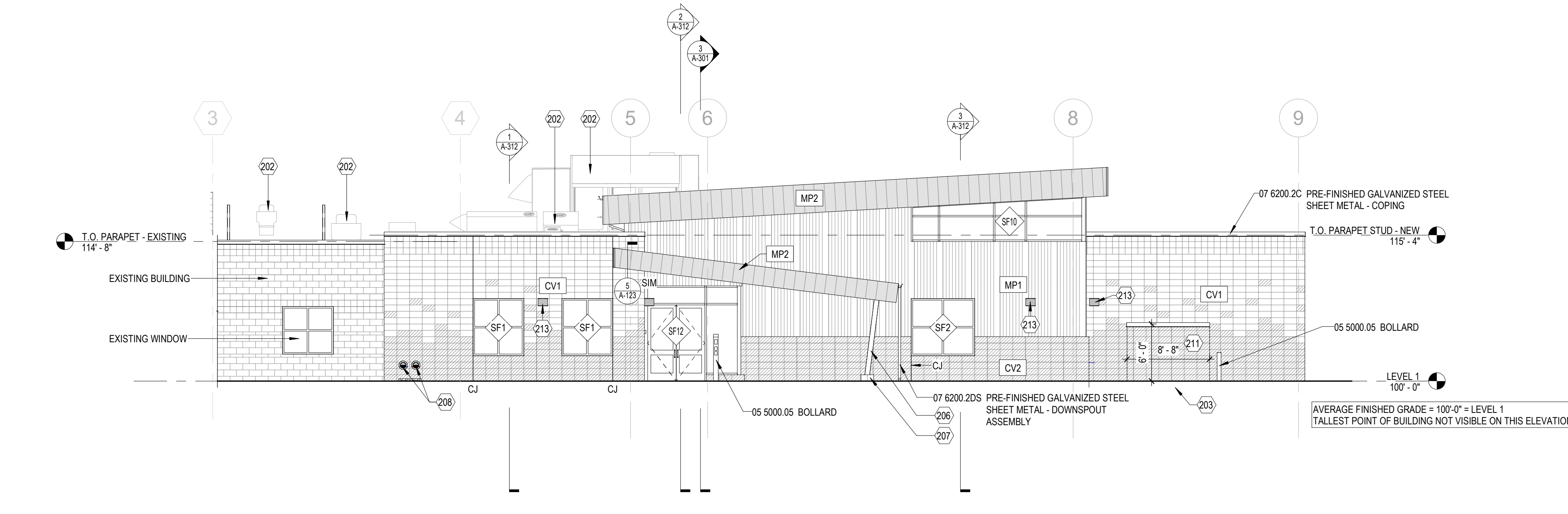
1 SOUTH ELEVATION 1/8" = 1'-0"
