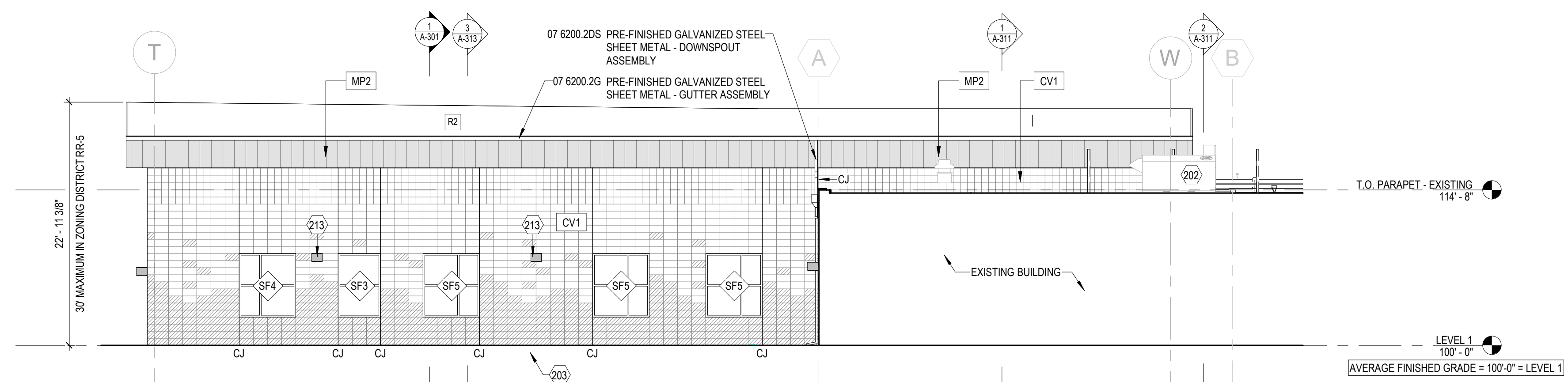
5 WEST ELEVATION 1/8" = 1'-0"
