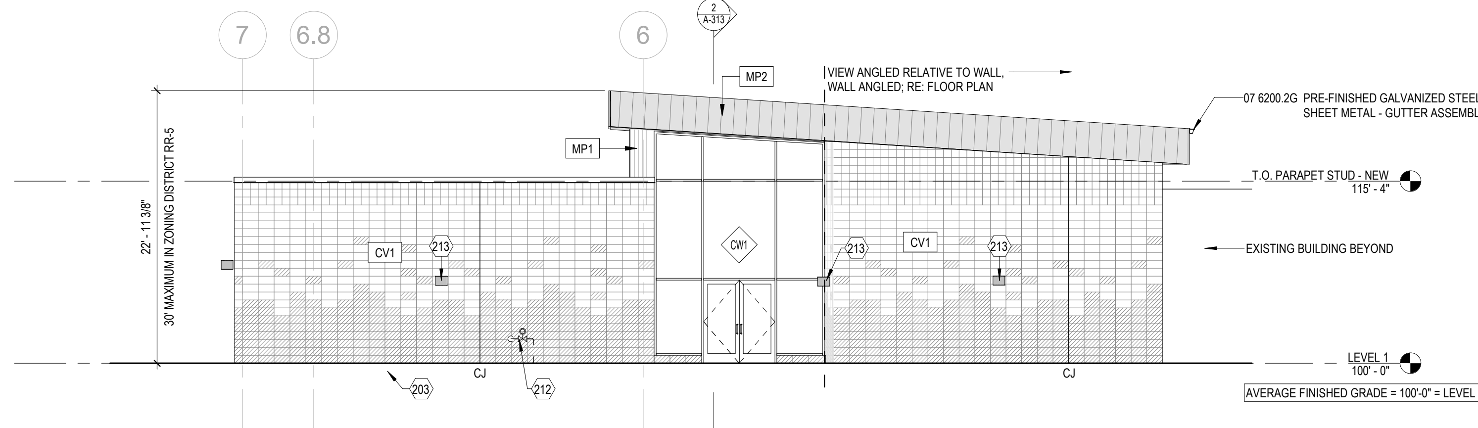
4 NORTH ELEVATION 1/8" = 1'-0"
