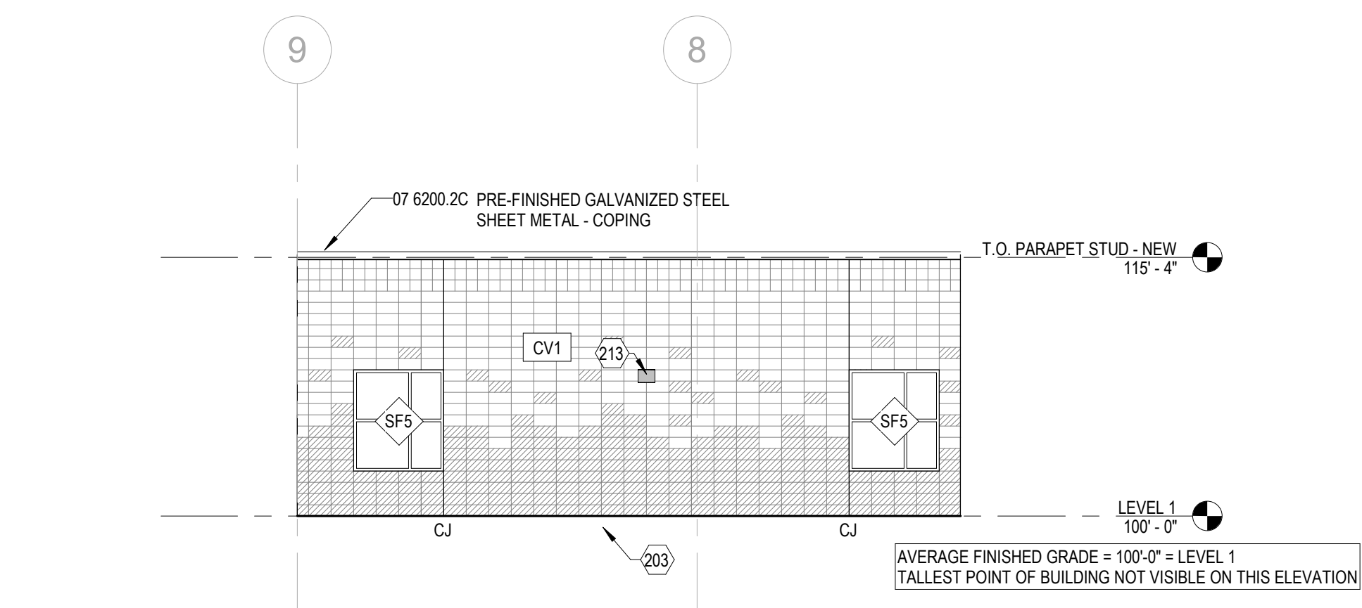
3 NORTH ELEVATION - OUTDOOR CLASSROOM 1/8" = 1'-0"
