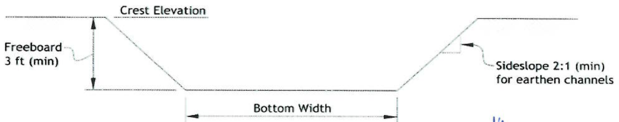
Spillway Section
