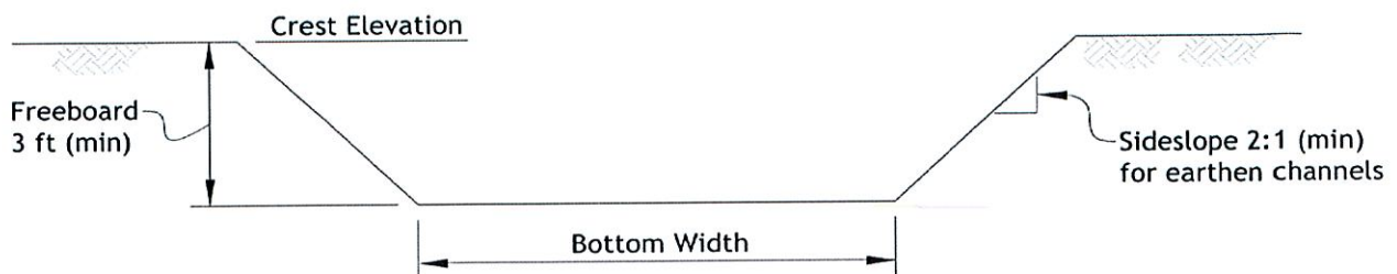
Spillway Section
