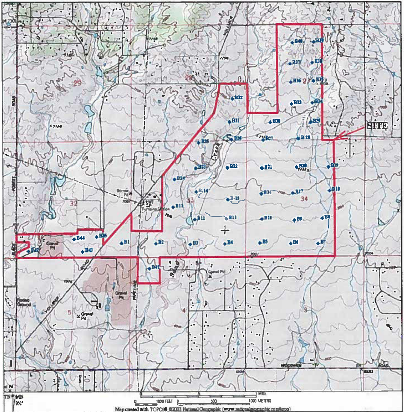
B1 - Approximate location of Test Borings
