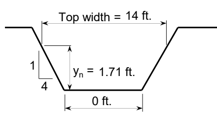
Inlet Channel Cross Section
