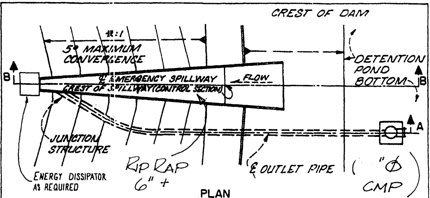
TYPICAL SPILLWAY AND OUTLET WORKS
