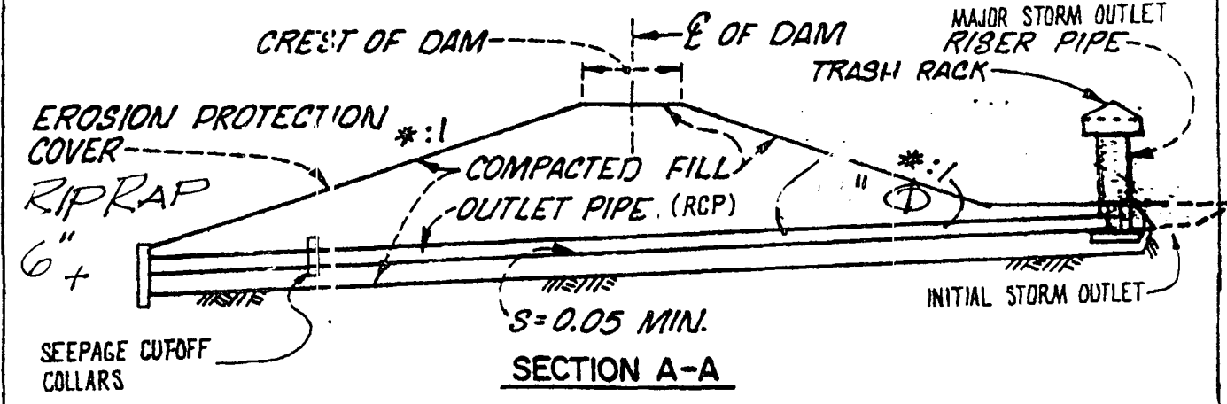
TYPICAL SPILLWAY AND OUTLET WORKS
