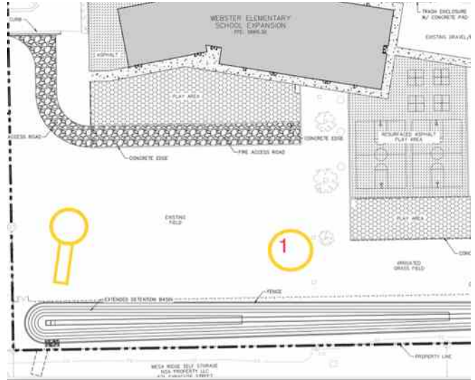
Yellow represents forebay and storm detention channel and red number represents test location
