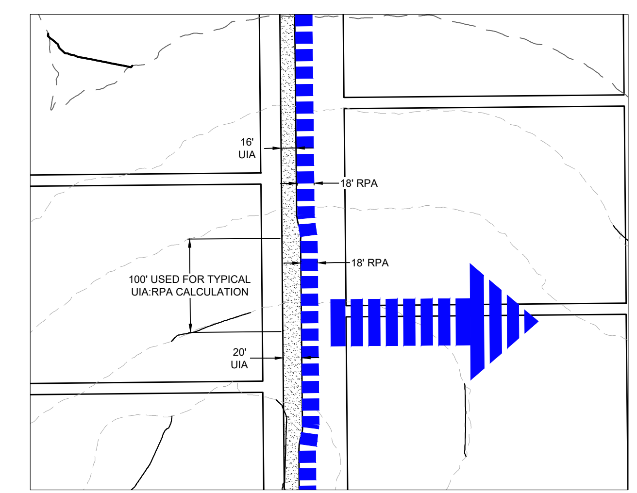
TYPICAL DETAIL
