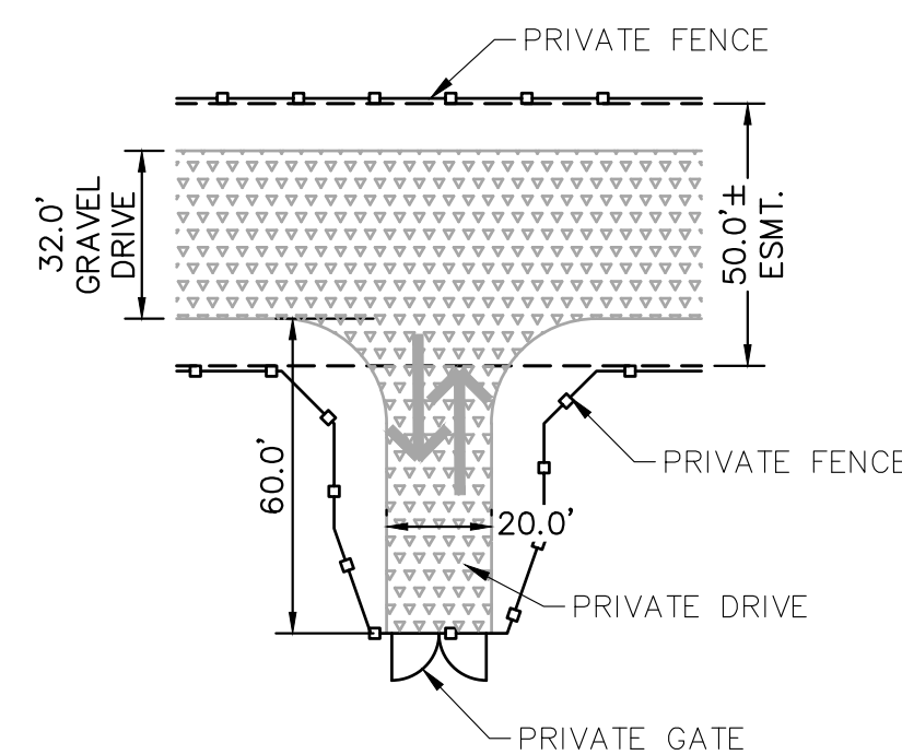
1 ALTERNATIVE HAMMERHEAD/Private Fence Layout Typical Turn Round
