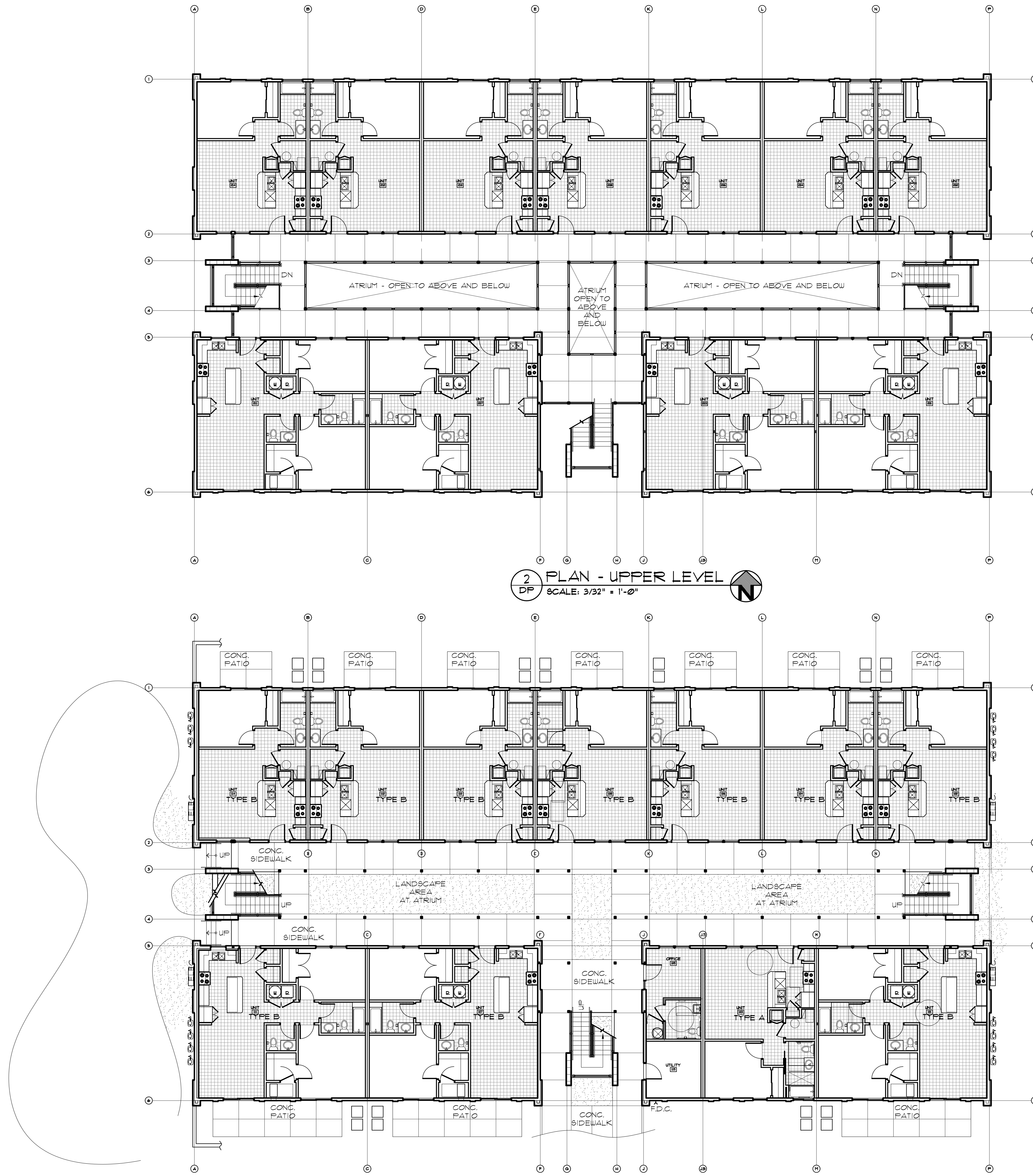
1 PLAN - MAIN LEVEL DP SCALE: 3/32" = 1'-0"
