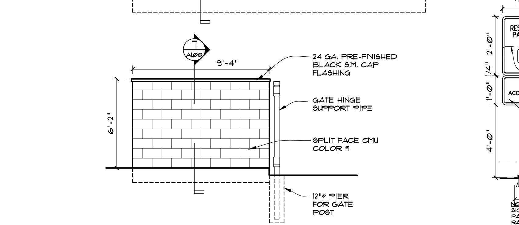
10 ELEVATION - TRASH ENCLOSURE A100 SCALE: 1/4" - 1'-0"
