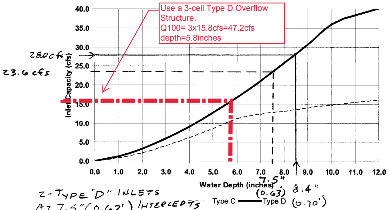
Allowable Inlet Capacity for Type C and D Inlets for Sump Conditions
