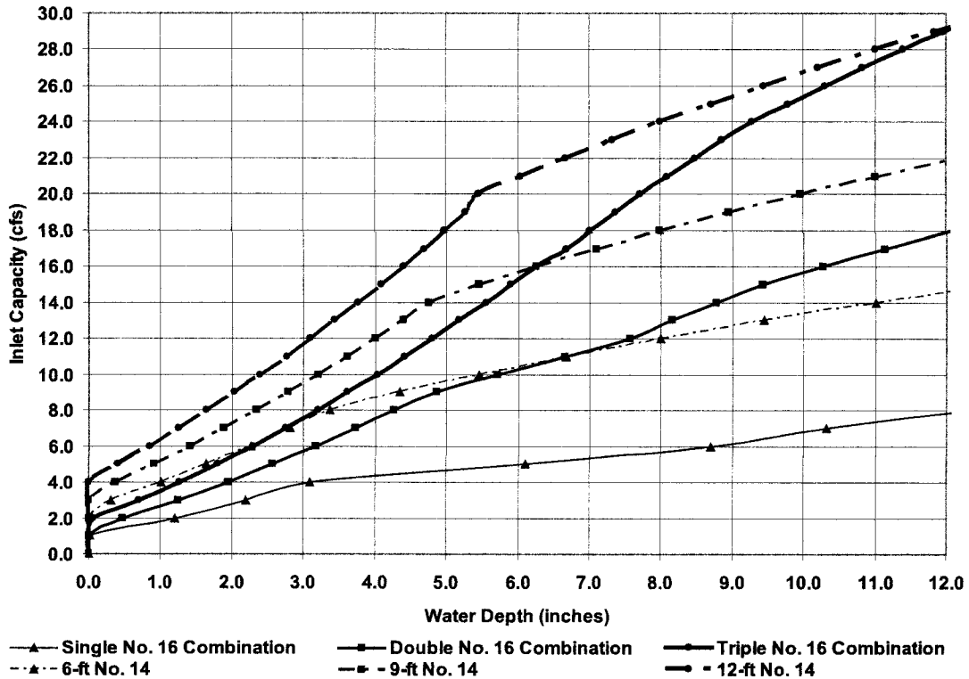
Allowable Inlet Capacity for Type C and D Inlets for Sump Conditions
