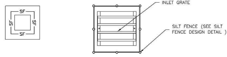
IP-4. SILT FENCE FOR SUMP INLET PROTECTION
