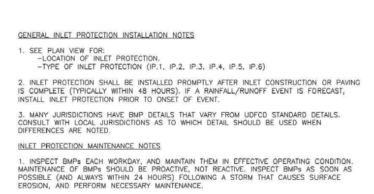
IP-8. INLET PROTECTION (IP)
