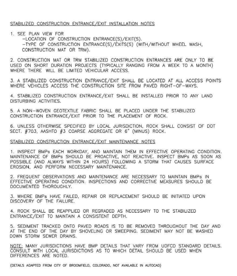
VTC-2. STABILIZED CONSTRUCTION ENTRANCE/EXIT INSTALLATION NOTES
