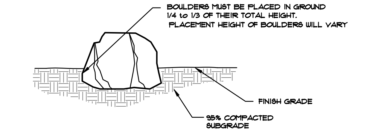
G ACCENT BOULDER SECTION NOT TO SCALE
