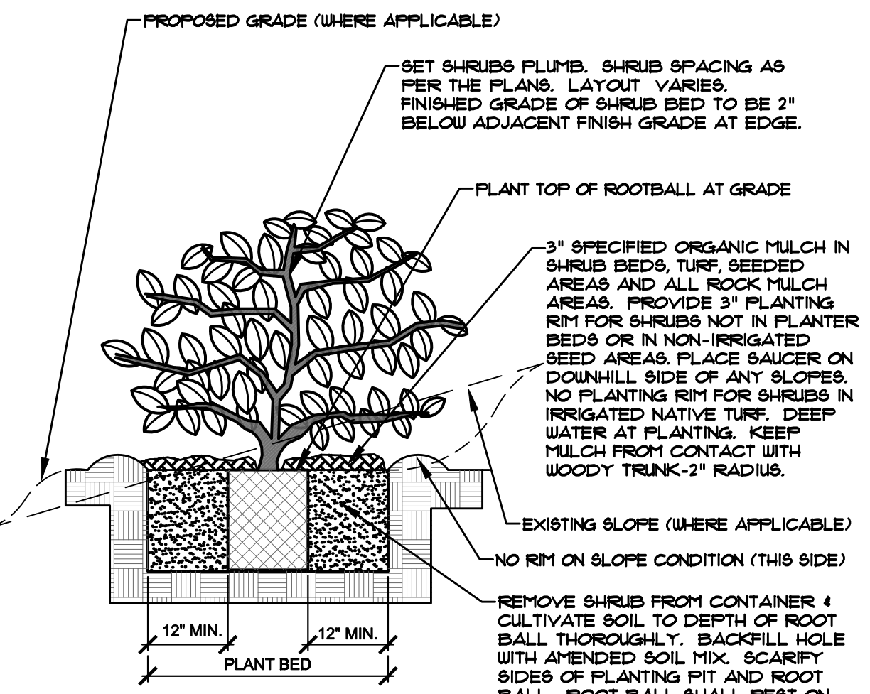
C SHRUB PLANTING DETAIL NOT TO SCALE
