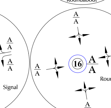
Figure 7b 2045 Background Lane Geometry, Traffic Control, and Levels of Service
