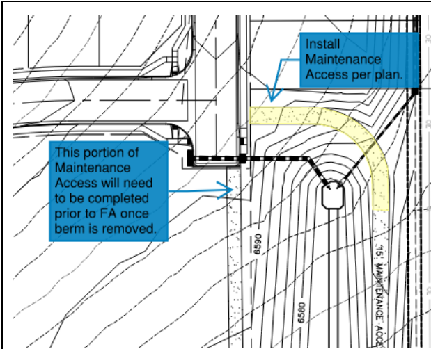
Photo 1: Install maintenance access road at NE end of South Pond per plan. A section of the western portion of the access road is incomplete due to a berm which is in place to protect the pond slopes. This section is not required to be completed prior to Preliminary Acceptance but will need to be installed prior to Final Acceptance.
