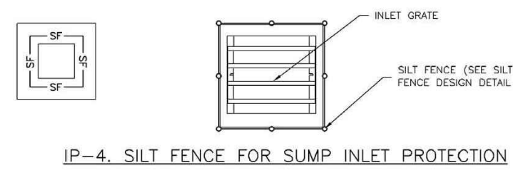
IP-4. SILT FENCE FOR SUMP INLET PROTECTION
