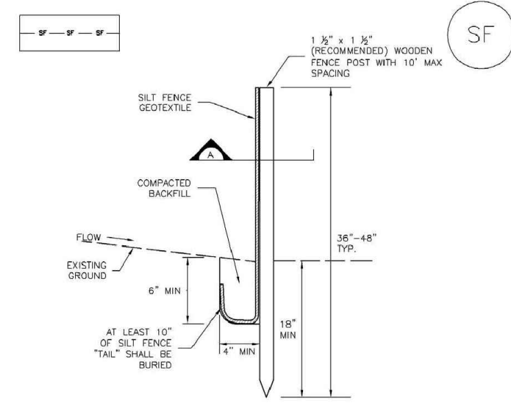
SILT FENCE
