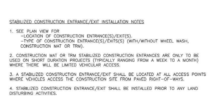
VTC-2. VEHICLE TRACKING CONTROL
