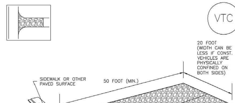
VTC-1. AGGREGATE VEHICLE TRACKING CONTROL
