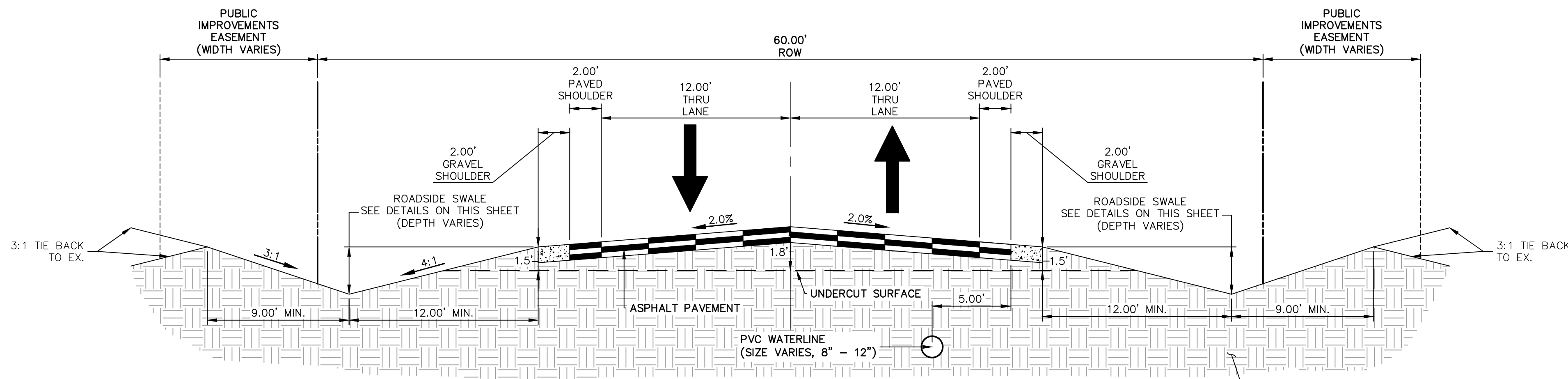
TYPICAL RURAL LOCAL POSTED SPEED LIMIT = 30 MPH, DESIGN SPEED LIMIT = 30 MPH SCALE: 1" = 5'
