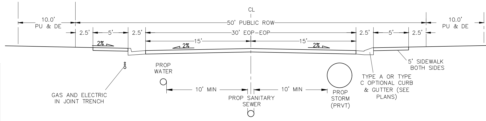
TYPICAL INTERNAL ACCESS ROADS PUBLIC 30' MAT N.T.S.
