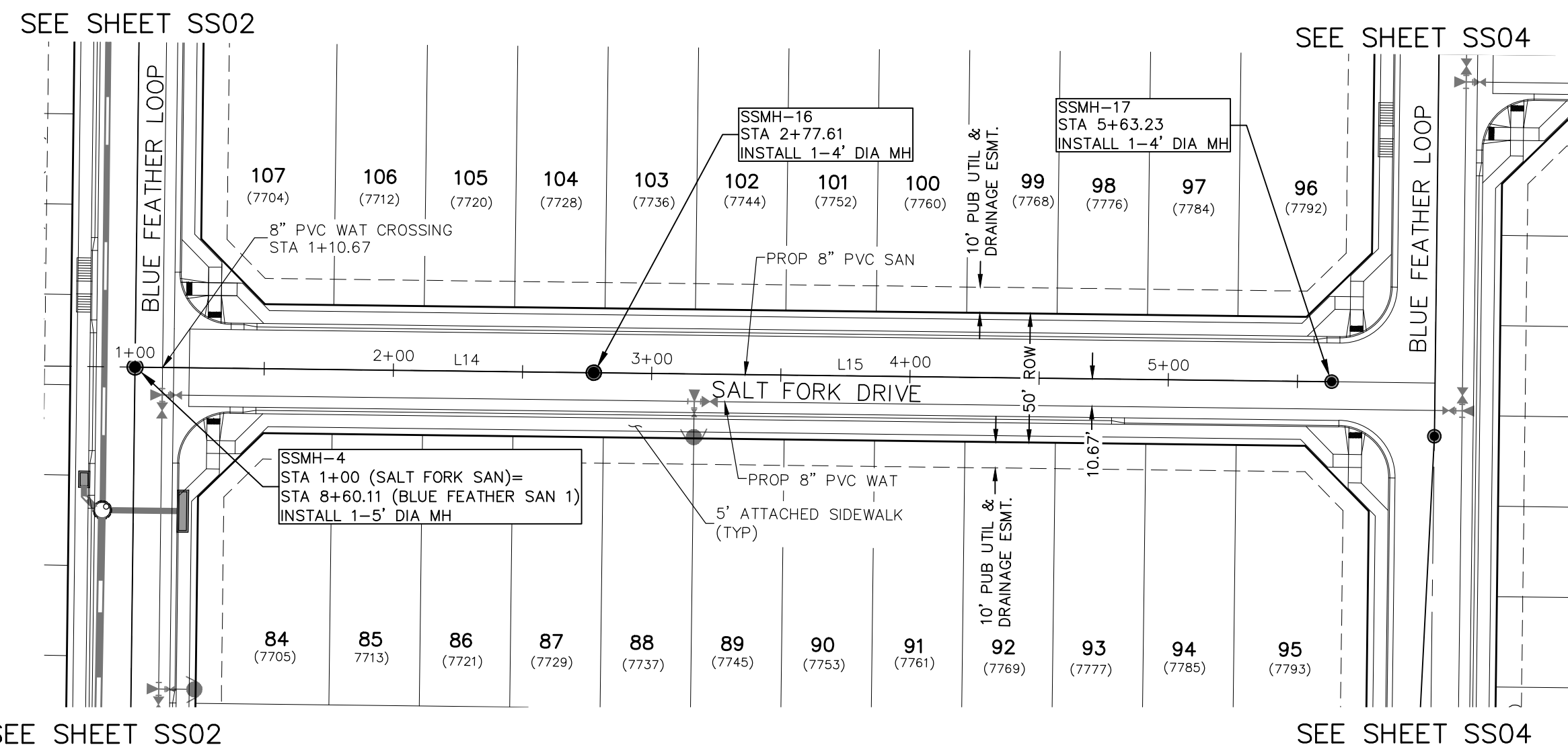
SALT FORK DRIVE SANITARY STA 1+00.00 TO STA 5+63.23
