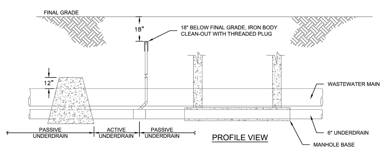
PASSIVE GROUNDWATER UNDERDRAIN SCHEMATIC
