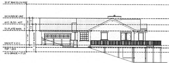
4 AVERAGE BUILDING HEIGHT 1/4" = 1'-0"
