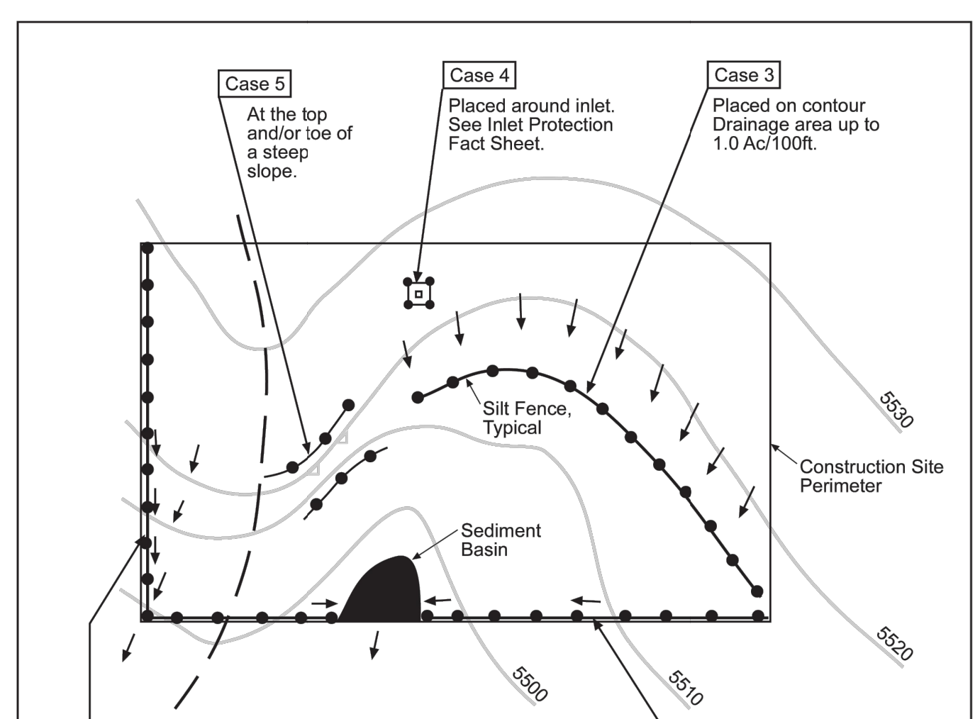
City of Colorado Springs Storm Water Quality Figure SF-1 Silt Fence Application Examples
