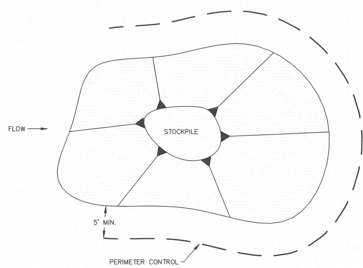
STOCKPILE PROTECTION PLAN
