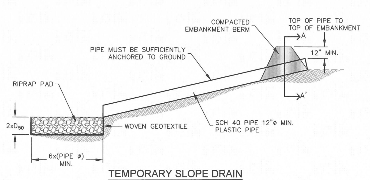
TEMPORARY SLOPE DRAIN
