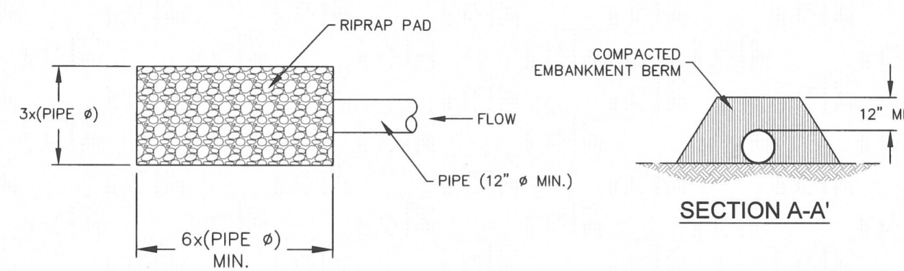
RIPRAP PAD PLAN
