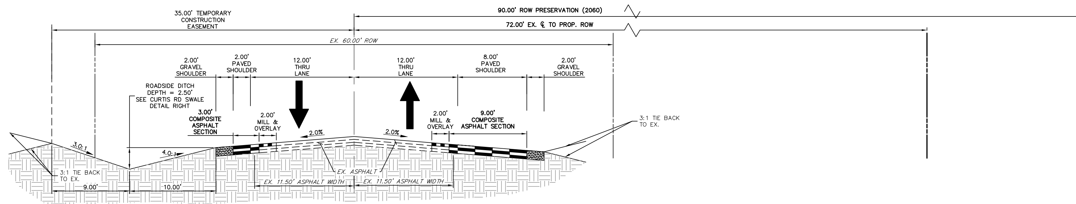
CURTIS ROAD - MODIFIED MINOR RURAL ARTERIAL - INTERIM FUTURE STA: 30+81.09-36+99.71 & 48+96.29-49+32.21 POSTED SPEED LIMIT = 45 MPH SCALE: 1" = 6' (LOOKING NORTH)
