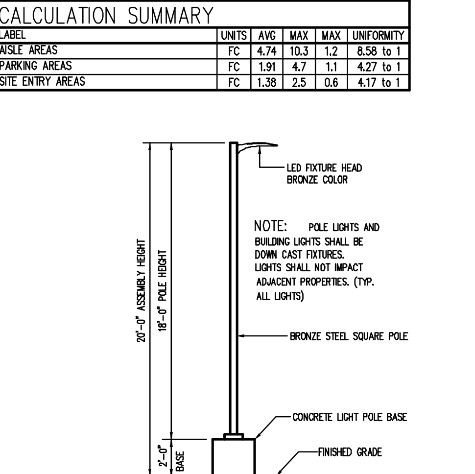
2 AREA LIGHT DETAIL SCALE: NOT TO SCALE
