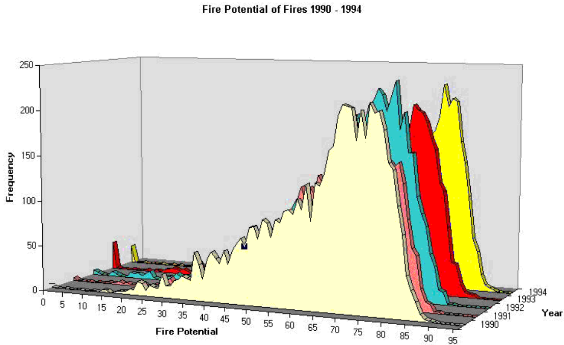
Figure 7. For only those pixels in which fires occurred, in the years 1990 to 1994, the frequency of FPI index values is shown.
