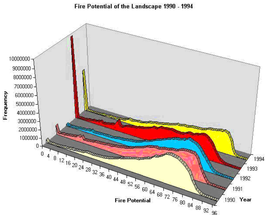
Figure 8. The frequency of pixels in the entire study area is shown for Fire Potential Index values calculated for 1990 to 1994.
