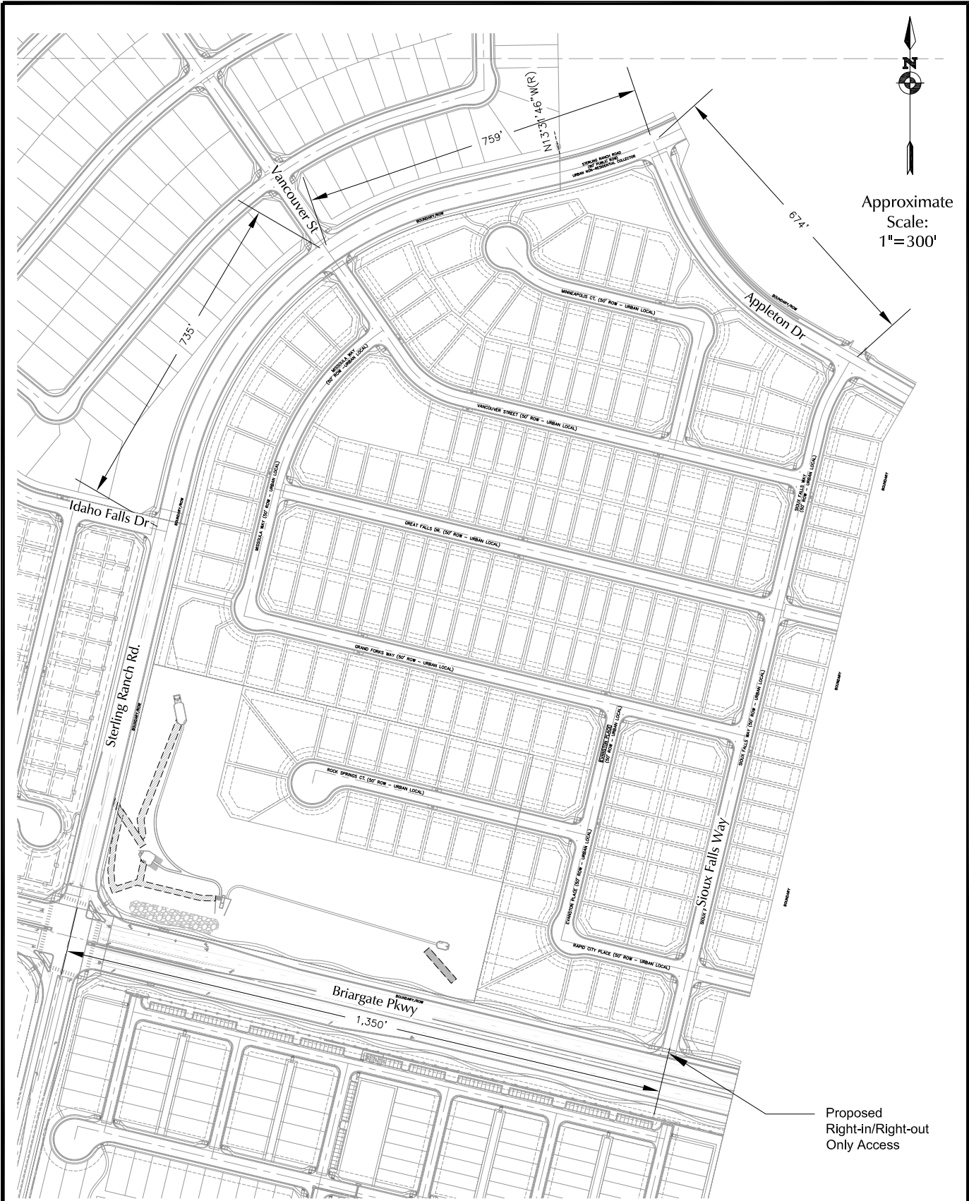
Figure 2 Site Plan
