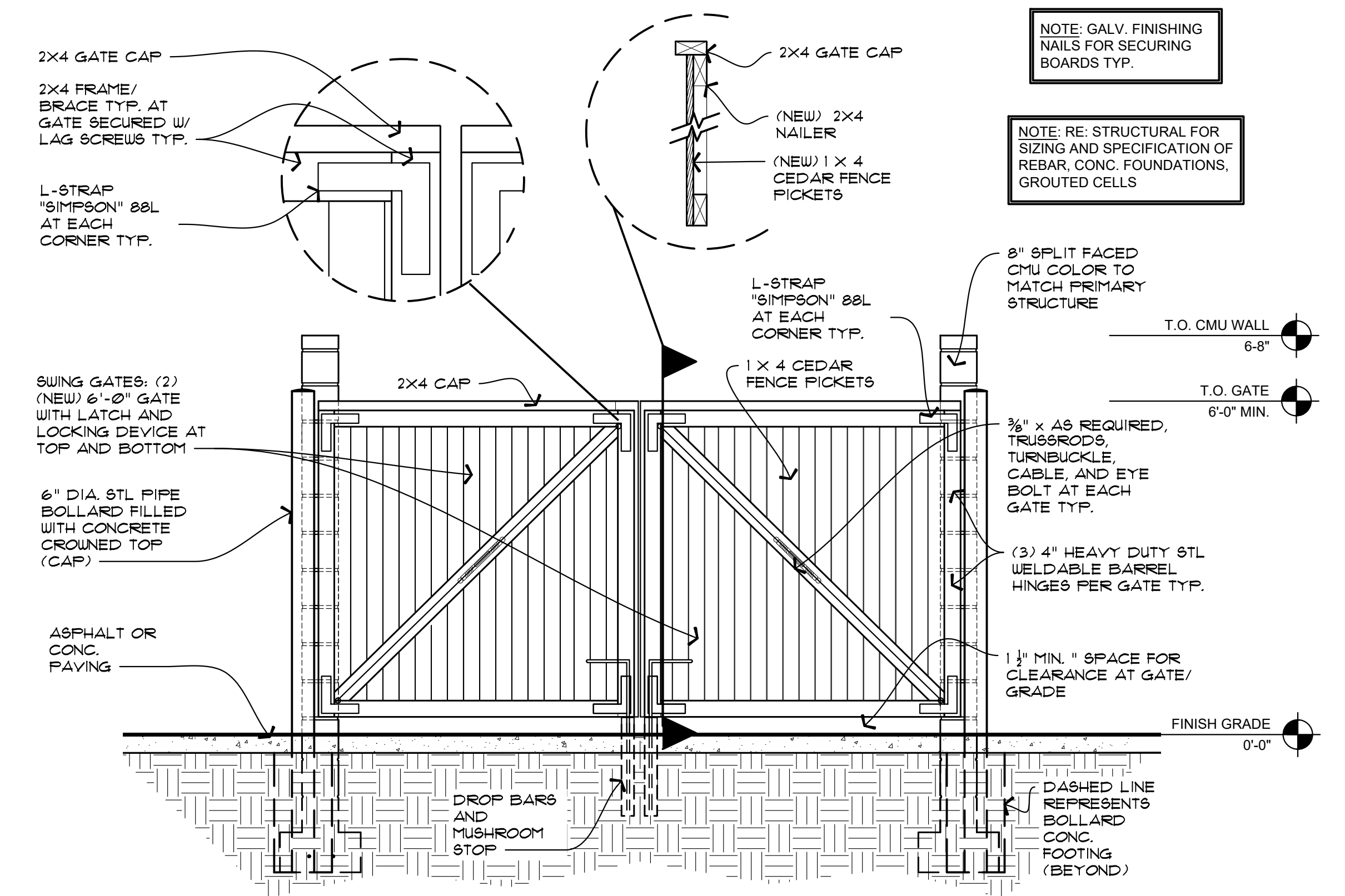
TRASH ENCLOSURE ELEVATION SCALE: 1/2" = 1'-0" 0" 1" 2" 4"
