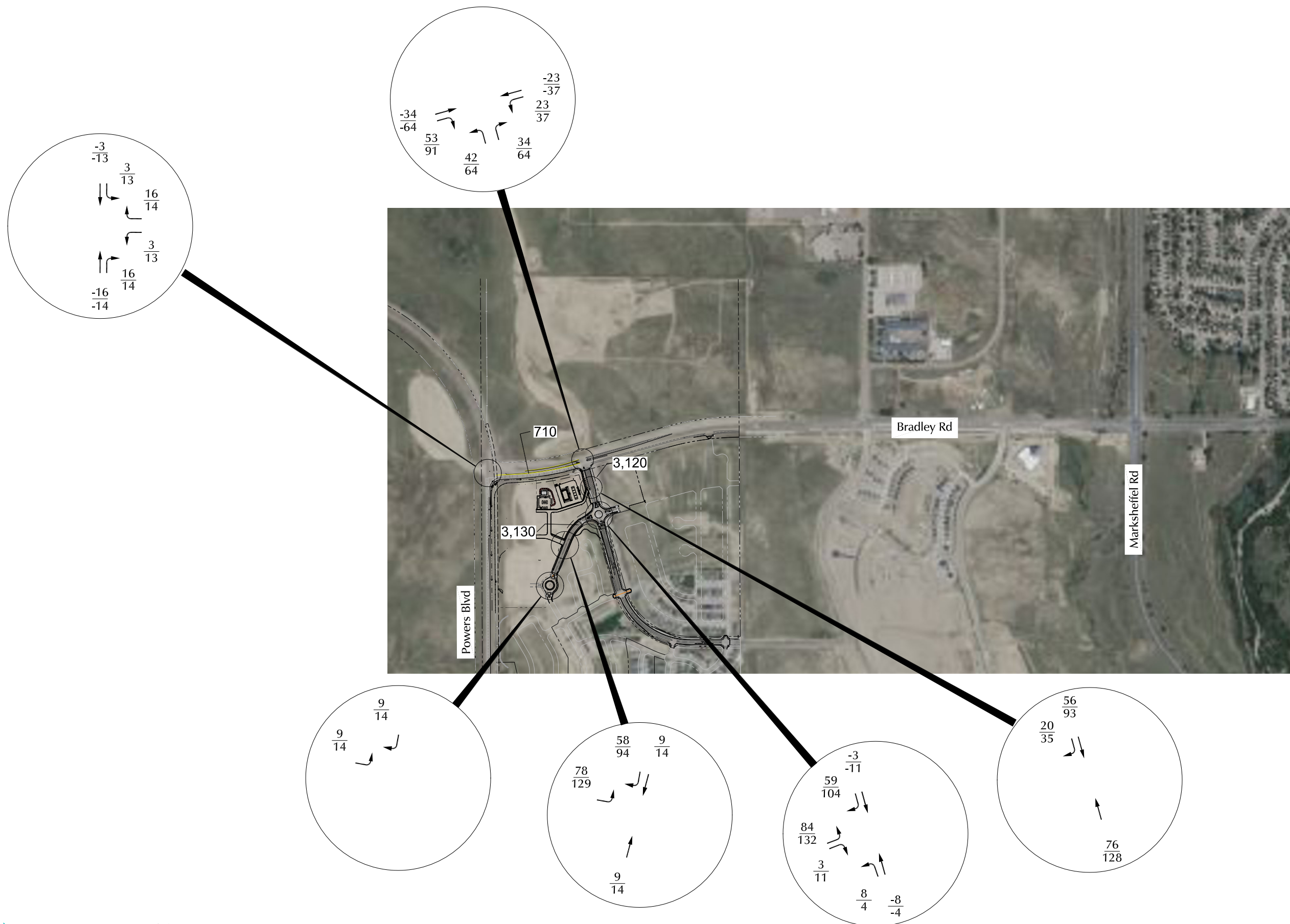
Pass-by Future Waterview East Commercial Filings-Generated Traffic
