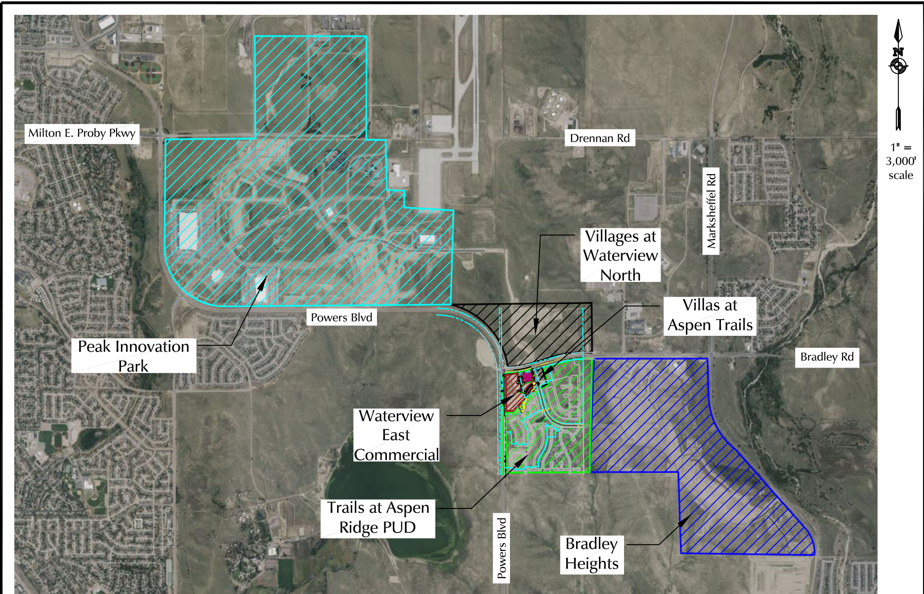
Figure 2 Context Map
