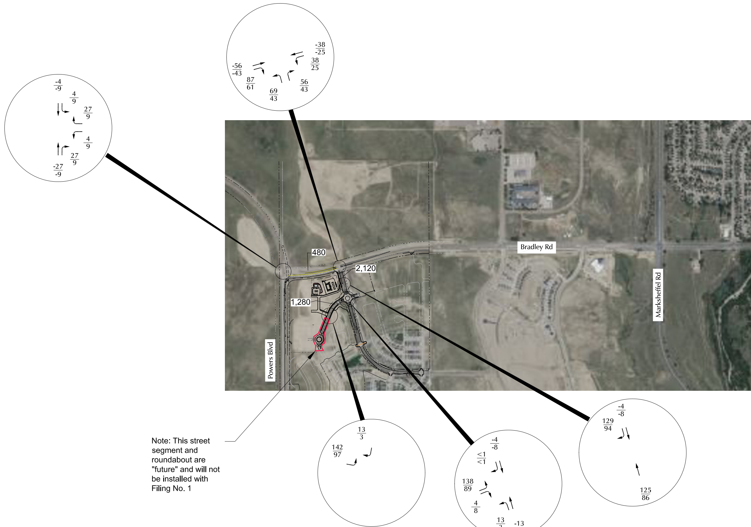
Figure 10a Pass-by Filing No. 1-Generated Traffic Waterview East Commercial Filing No. 1 (LSC #S214971)
