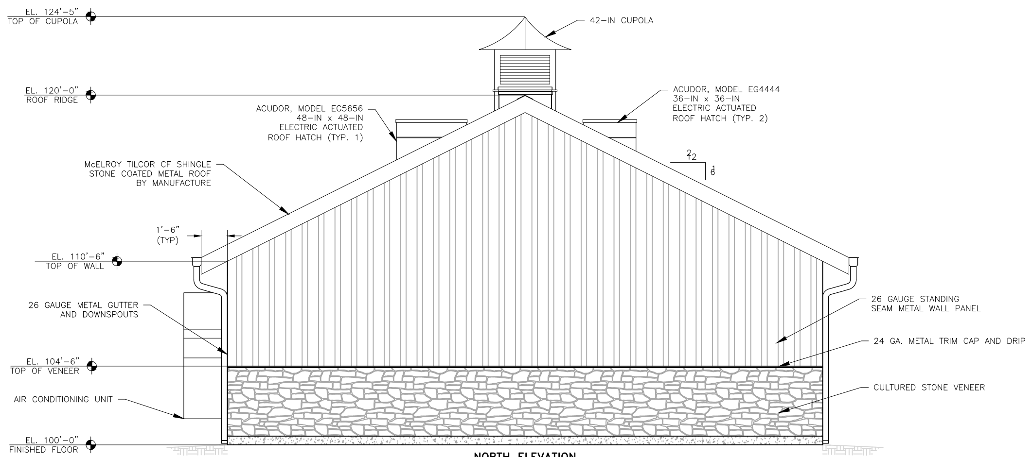
NORTH ELEVATION SCALE: 3/16" = 1'0"
