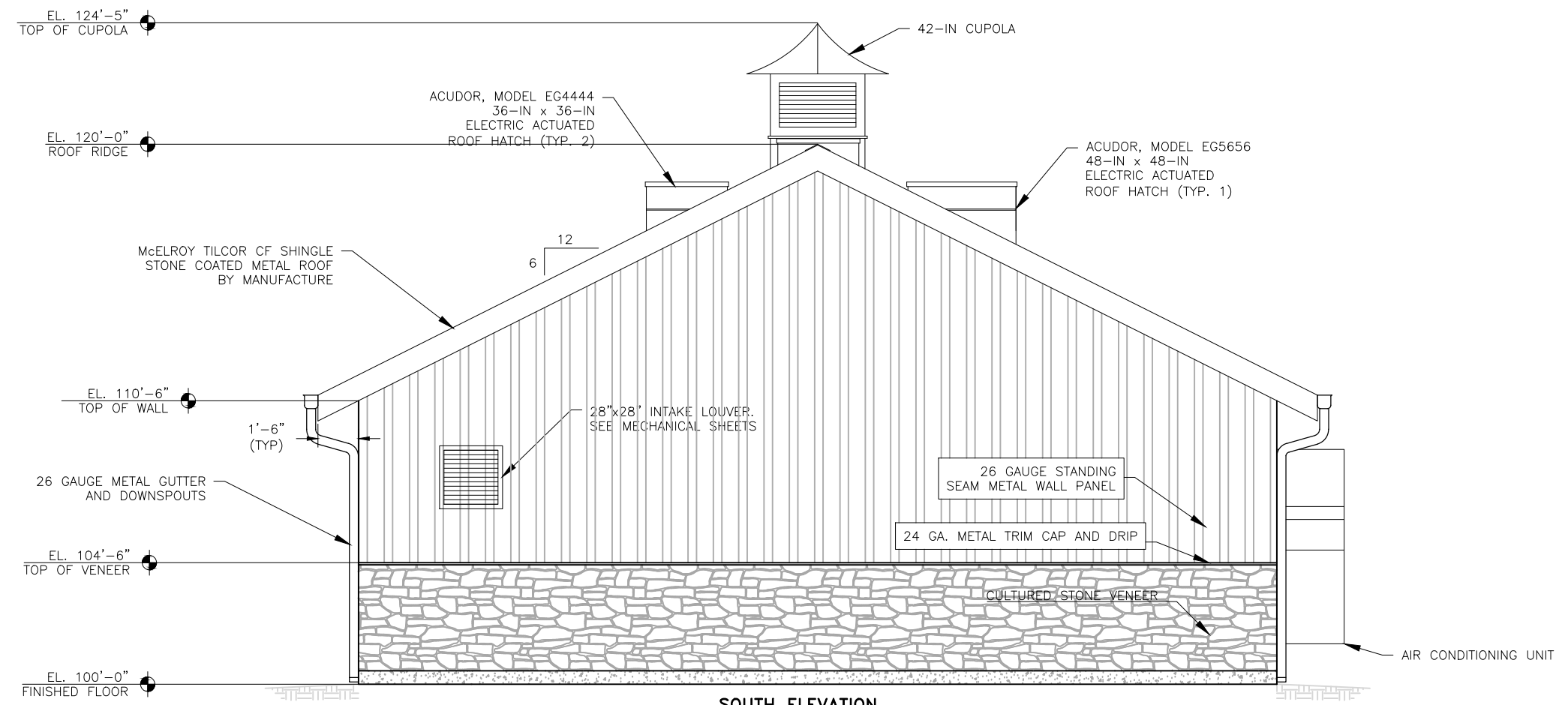
SOUTH ELEVATION SCALE: 3/16" = 1'0"
