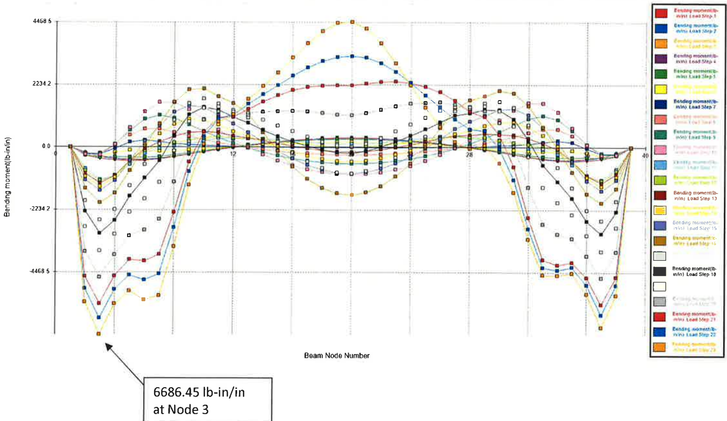
Bending moment(lb-in/in): Load steps 1,2,3,4,5,6,7,8,9,10,11,12,13,14,15,16,17,18,19,20,21,22,23,
