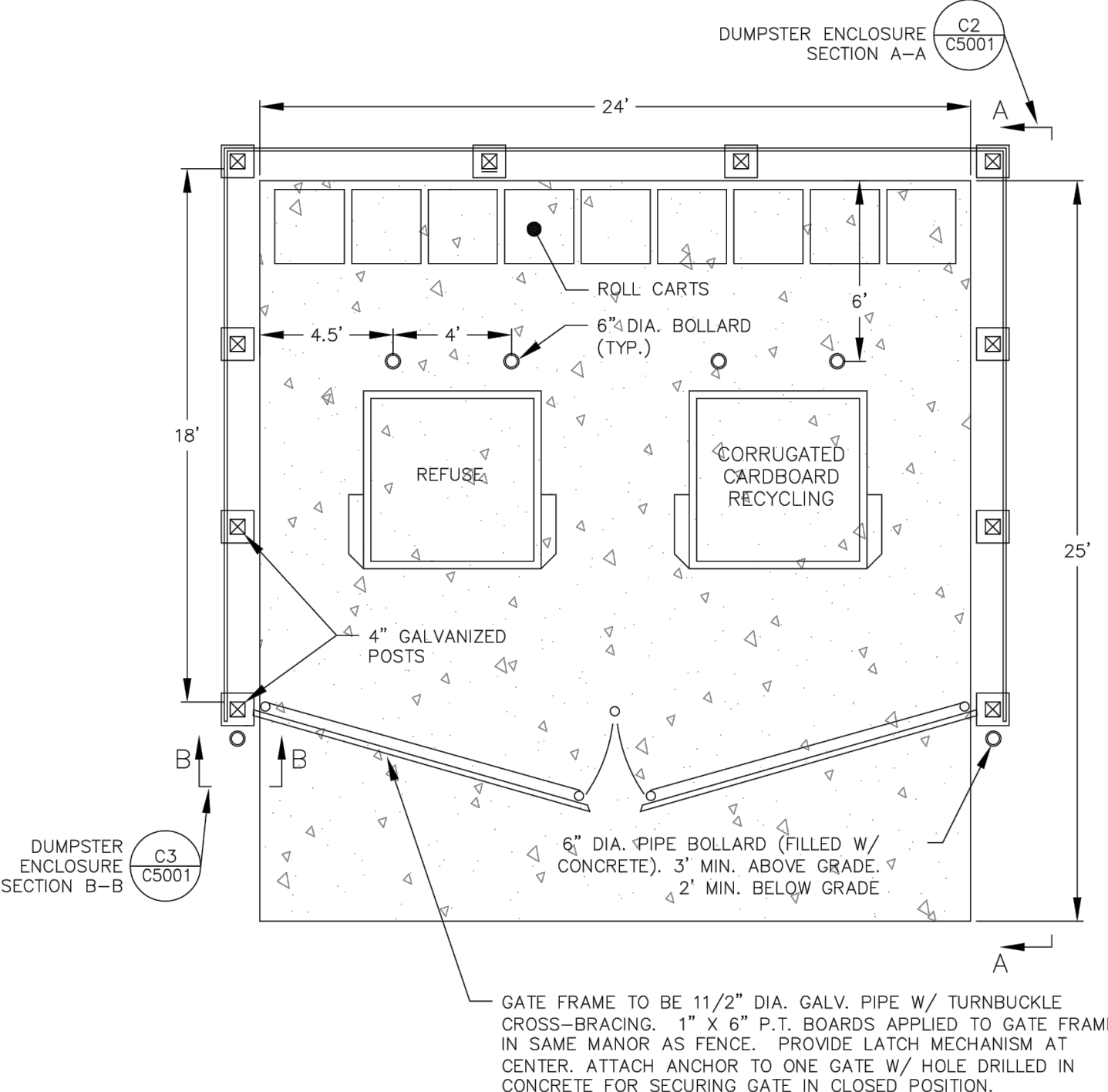
TRASH ENCLOSURE DETAIL NTS
