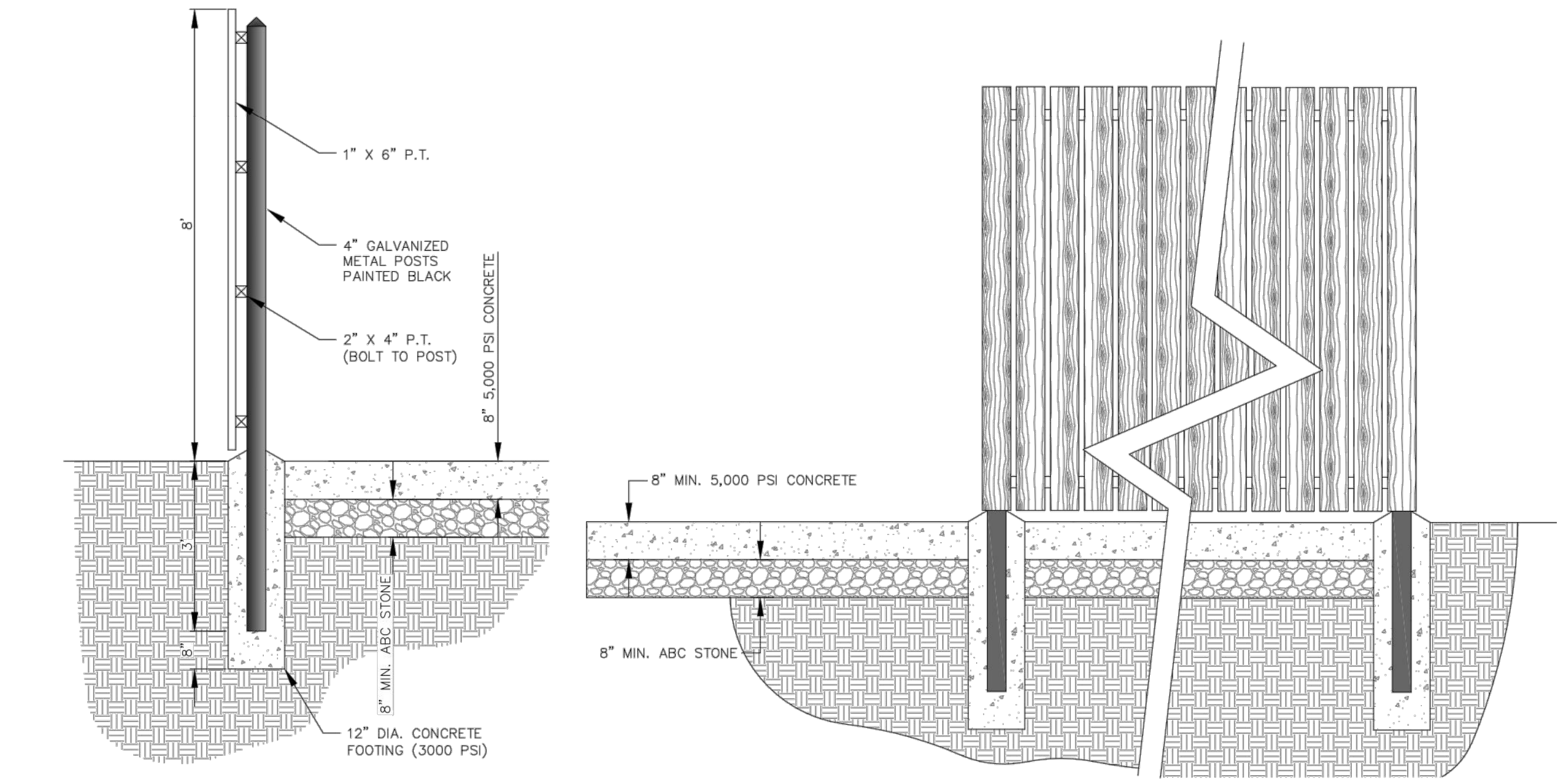
TRASH ENCLOSURE ELEVATIONS NTS
