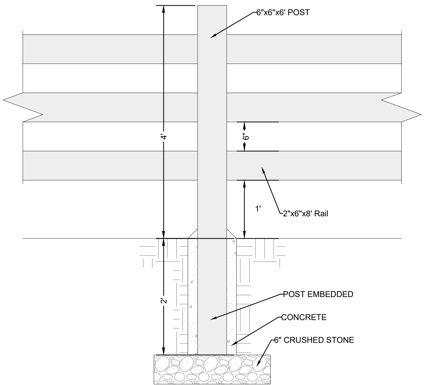
SPLIT RAIL FENCE DETAIL NTS
