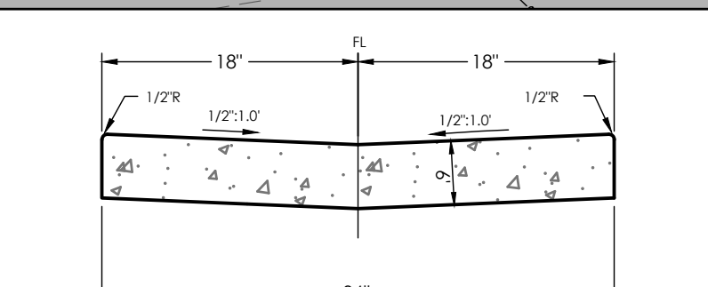
3' CONCRETE DRAIN PAN DETAIL SCALE 1" = 12"
