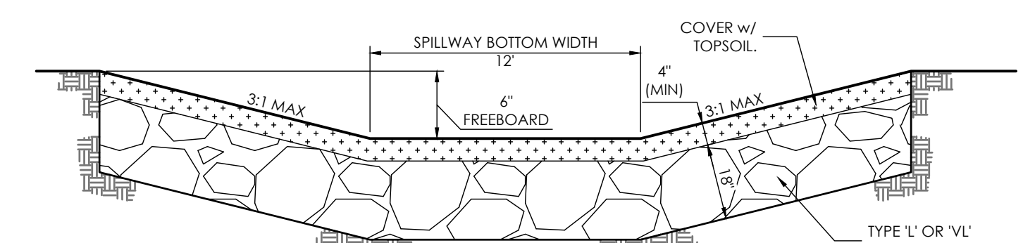
PHASE-II RAIN GARDEN SPILLWAY DETAIL SCALE: NTS
