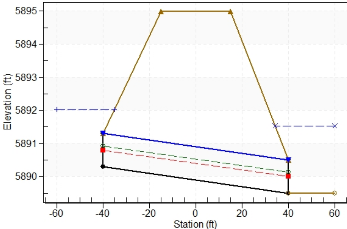
Crossing - Drennan Road Crossing, Design Discharge - 100.0 cfs Culvert - EX. 12-inch CMP, Culvert Discharge - 1.4 cfs
