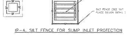
IP-4. SILT FENCE FOR SUMP INLET PROTECTION
