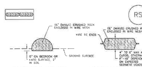
RS-1. ROCK SOCK PERIMETER CONTROL
