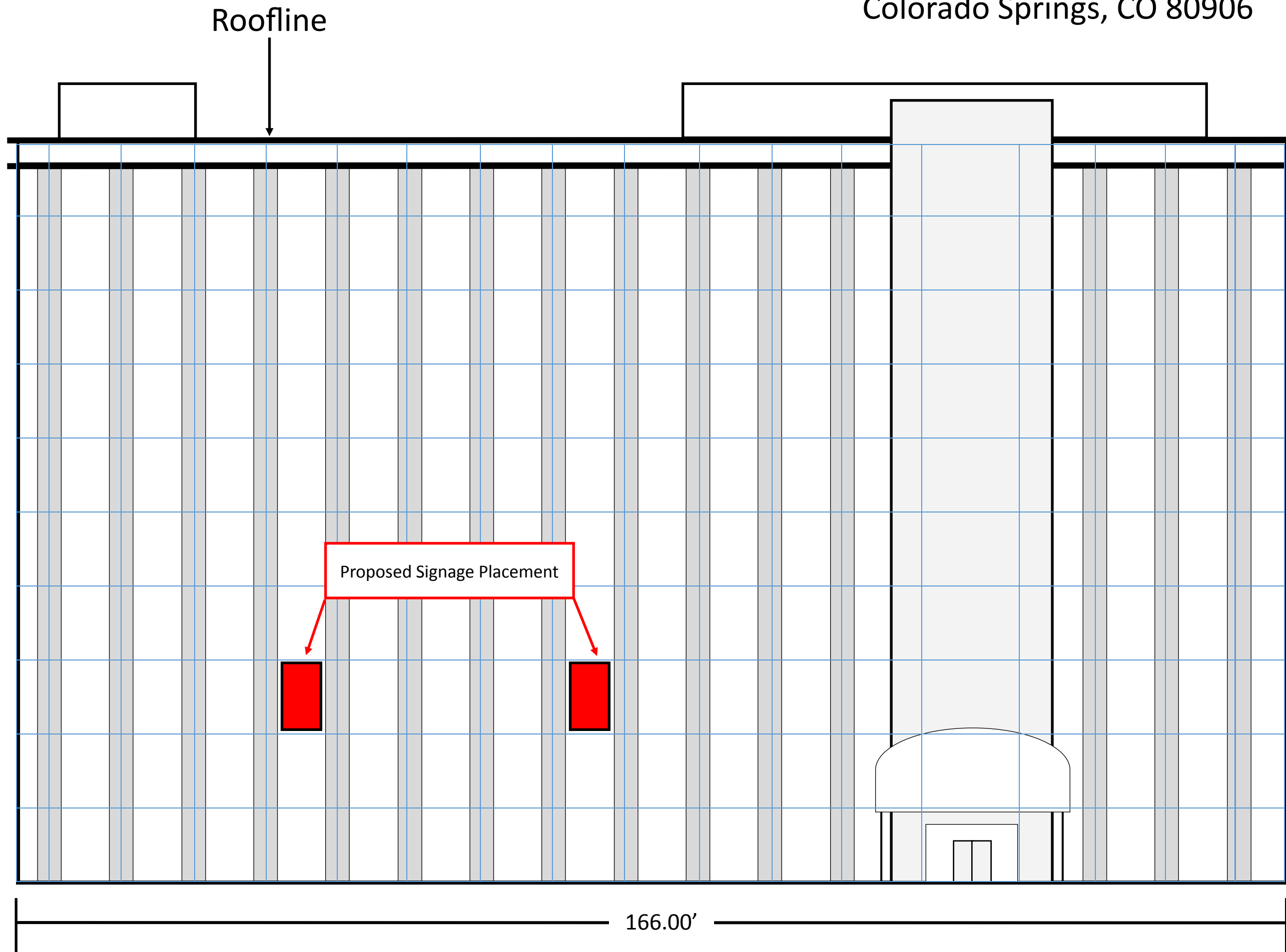
FRONT ELEVATION
