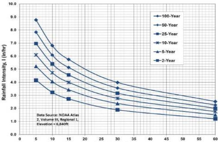
Figure 6-5. Colorado Springs Rainfall Intensity Duration Frequency
