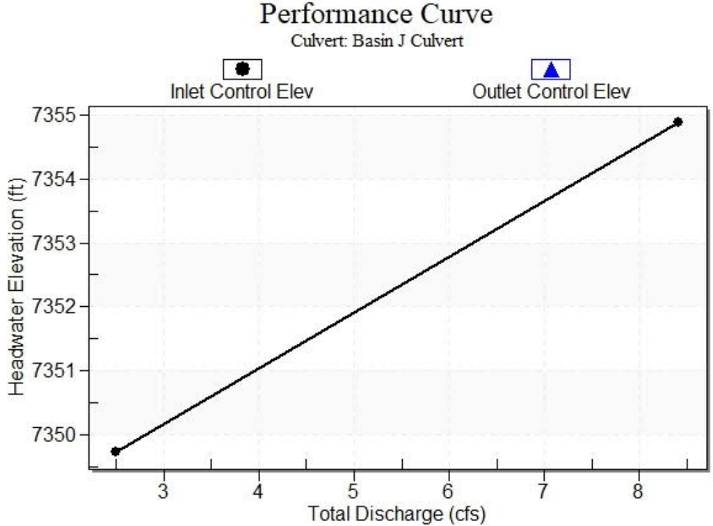
Culvert Performance Curve Plot: Basin J Culvert
