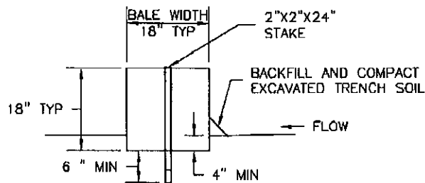
SECTION A
