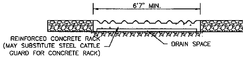
SECTION A
