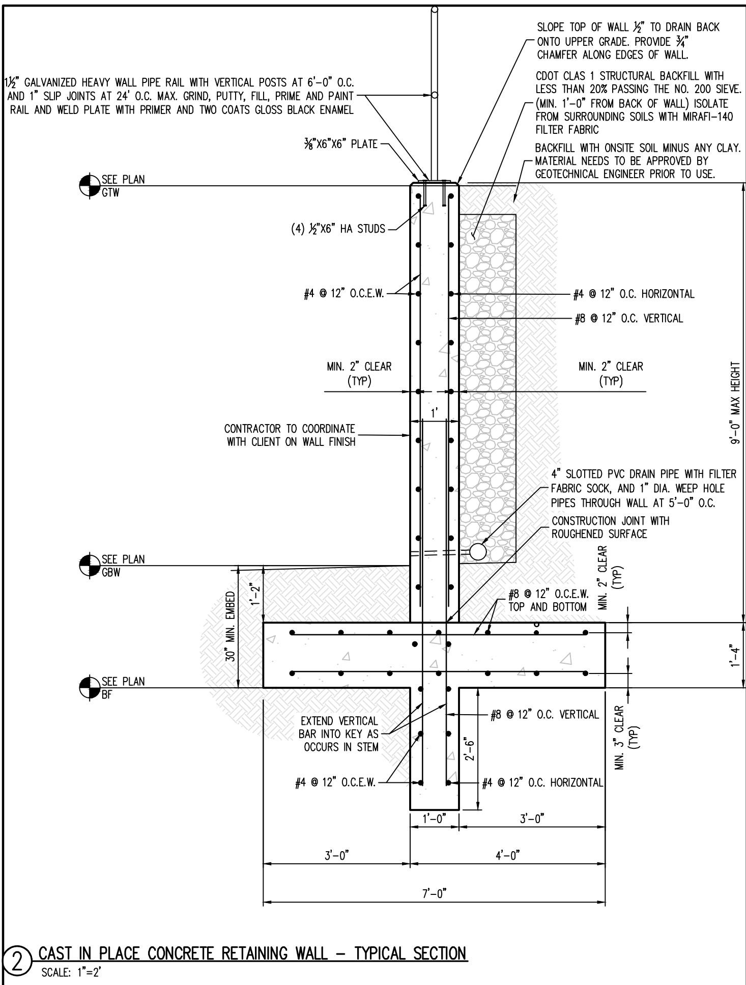
1 CAST IN PLACE CONCRETE RETAINING WALL - TYPICAL SECTION SCALE: 1"=2'
