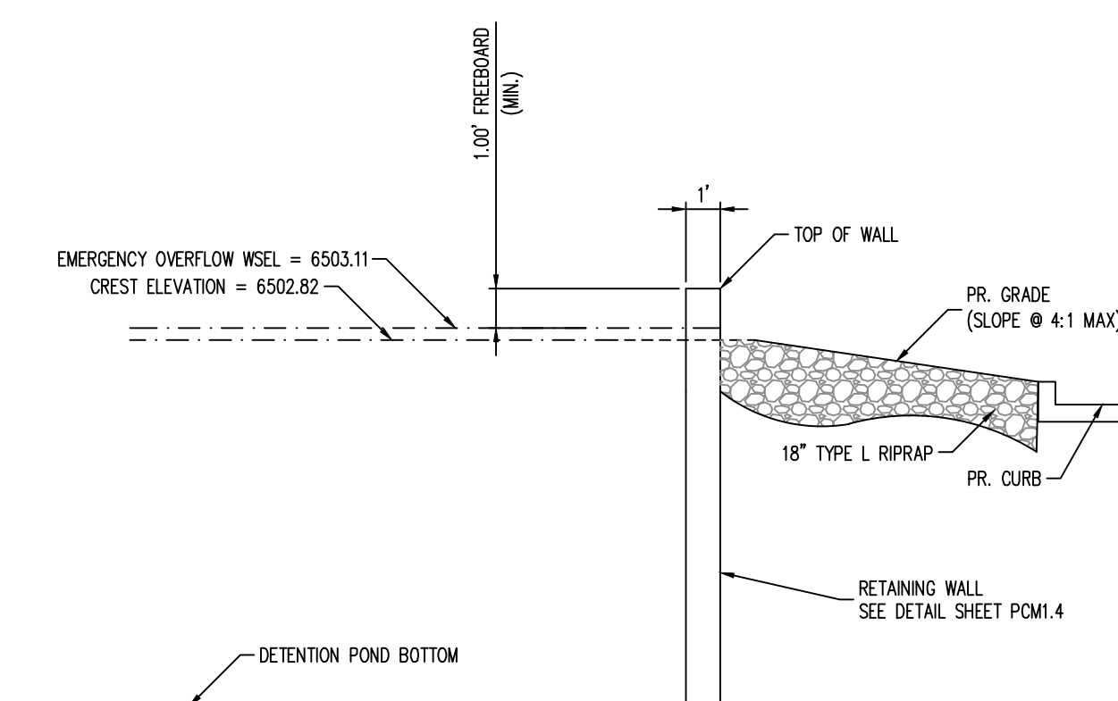
3 POND 100-YEAR OVERFLOW - PROFILE NOT TO SCALE
