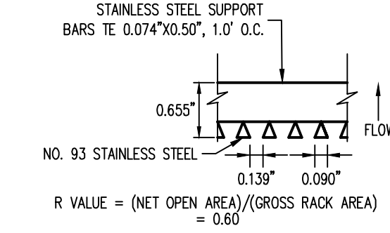
TRASH RACK SECTION SCALE: 1" = 1'
