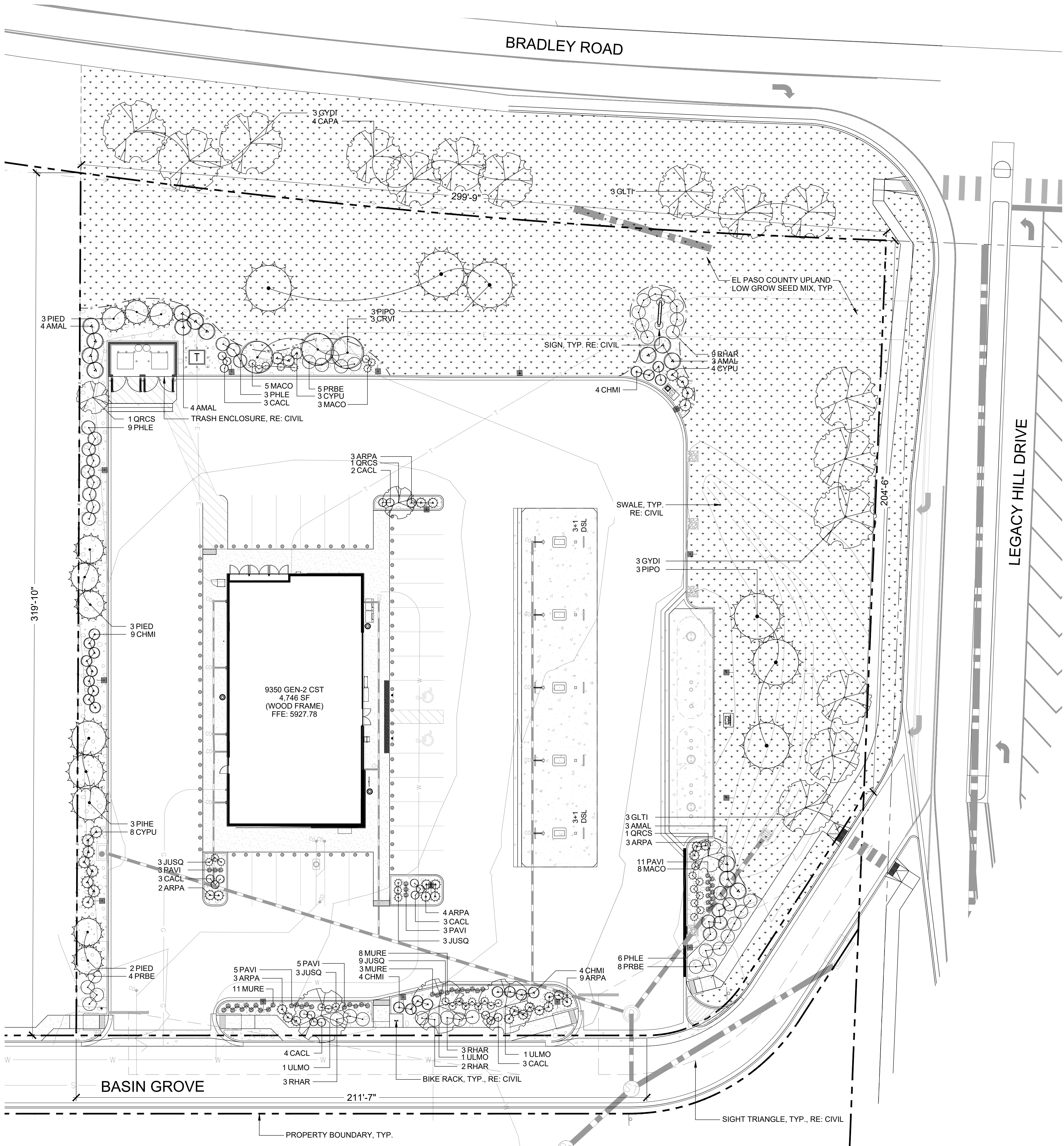
1 LANDSCAPE PLAN
