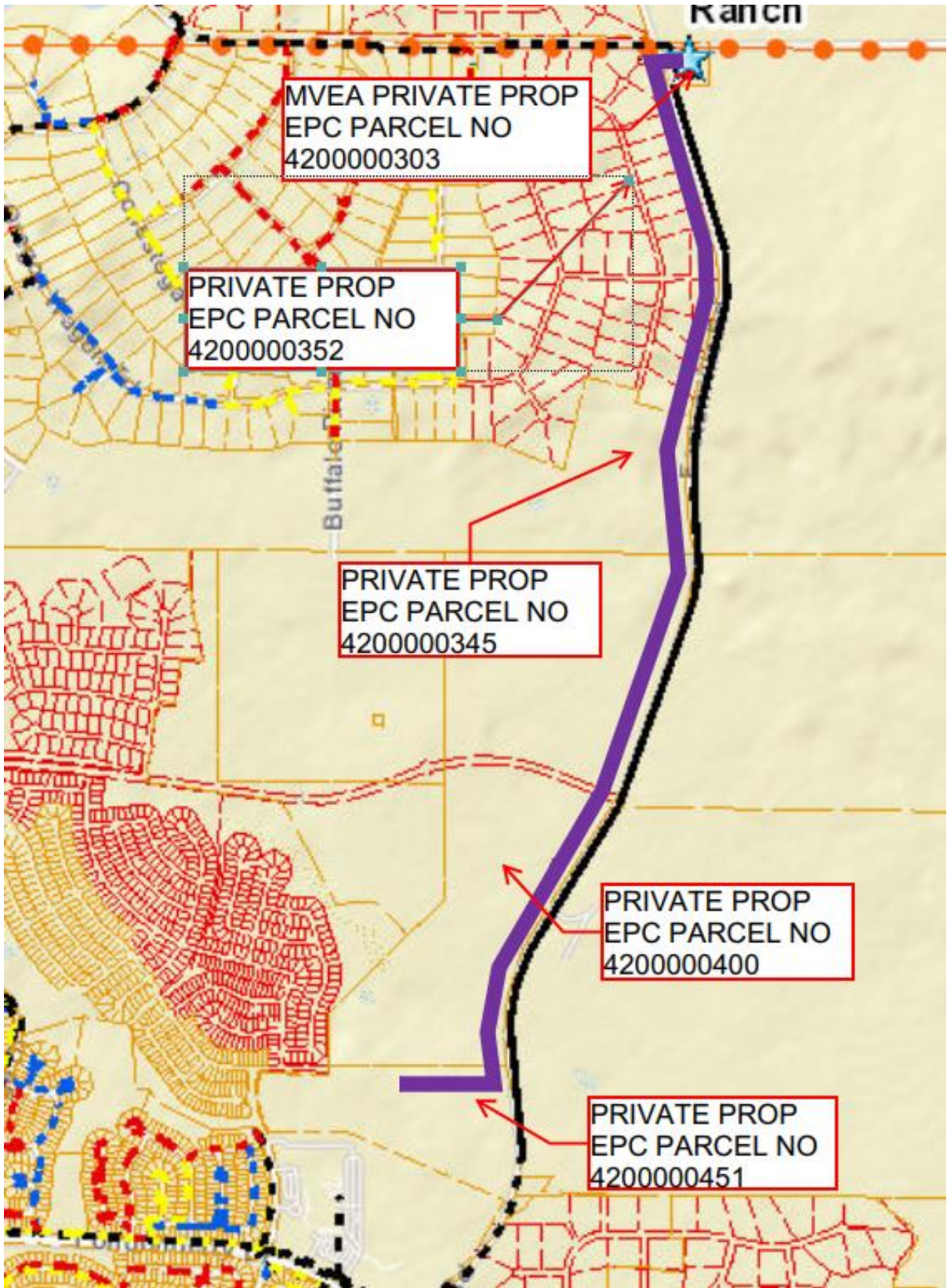
MVEA Eastonville II - MVEA System Map New (12.5 kv) Distribution Line (shown in purple)
