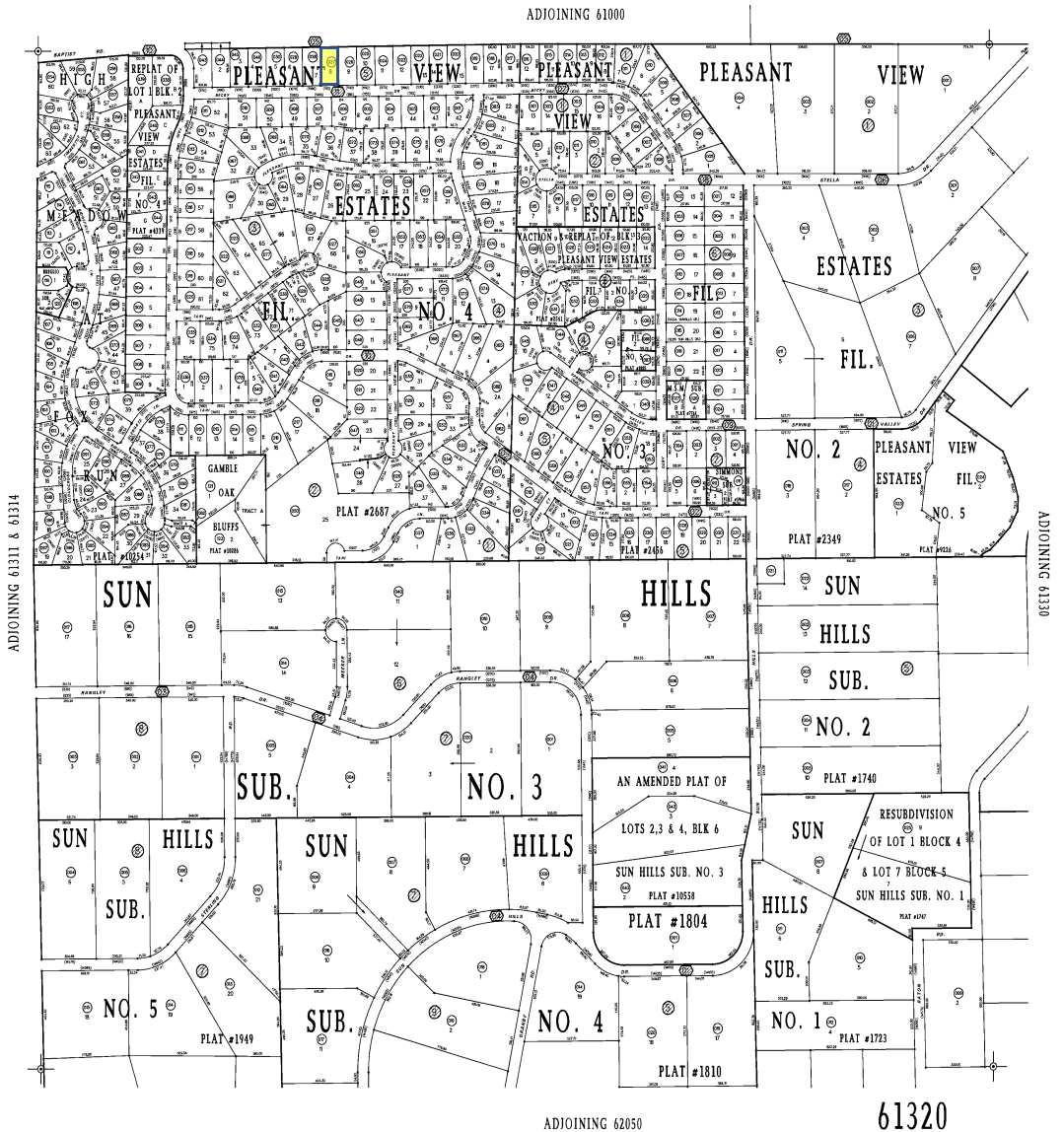
Rectangular Survey of One Section
