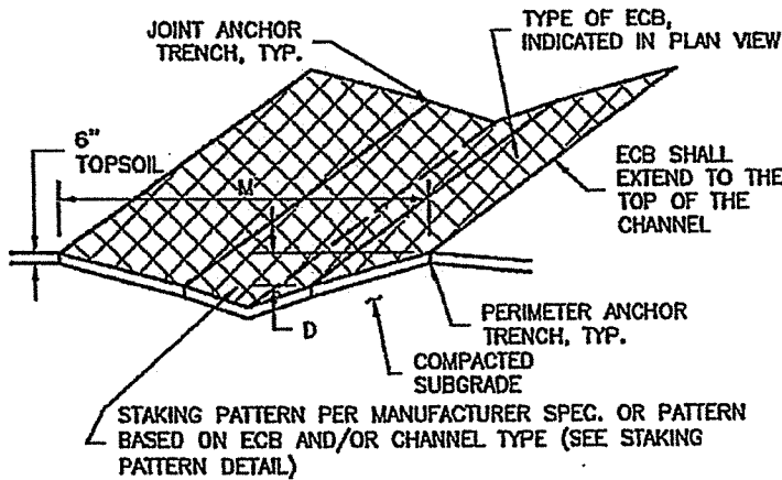
ECB-2. SMALL DITCH OR DRAINAGEWAY
