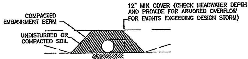
SECTION A
