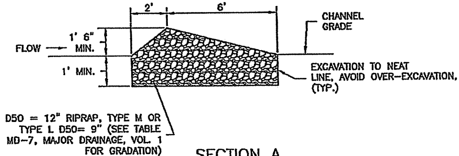
SECTION A
