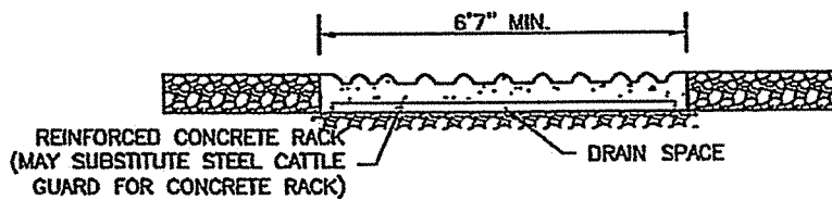
SECTION A
