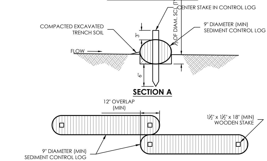
SECTION A SCL-1. SEDIMENT CONTROL LOG JOINTS
