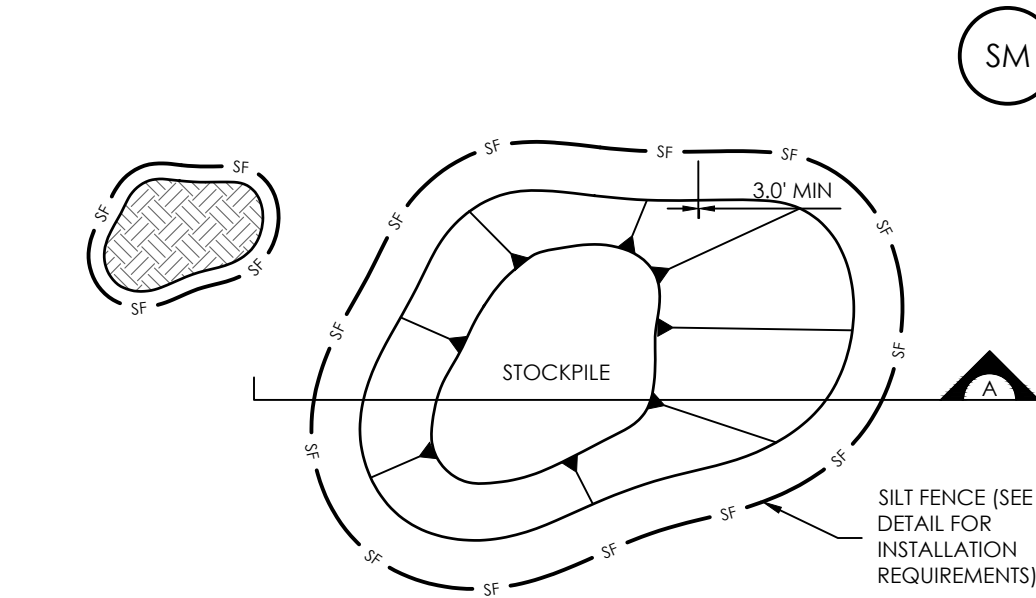
SECTION A SP-1. STOCKPILE PROTECTION
