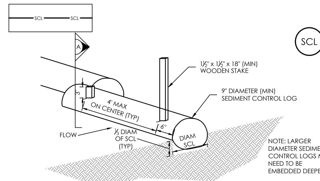
SECTION A SCL-1. SEDIMENT CONTROL LOG
