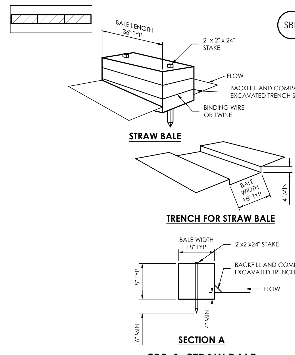
SECTION A SBB-1. STRAW BALE
