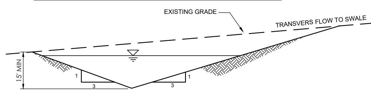
DS-1. COMPACTED UNLINED EXCAVATED SWALE
