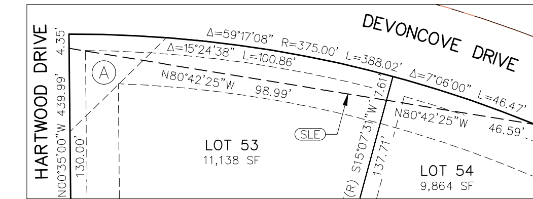
LOTS 53-54 SIGHT-LINE EASEMENT DETAIL SEE SHEET 8 SCALE: 1" = 30'
