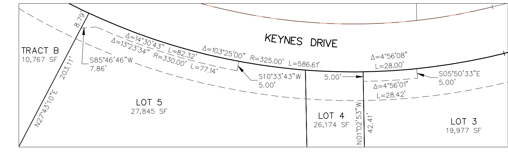
LOTS 3 AND 5 EASEMENT DETAIL STORM SYSTEM AND DRAINAGE SCALE: 1" = 30' 5 FOOT SIDE AND FRONT LOT LINE EASEMENTS NOT SHOWN FOR CLARITY
