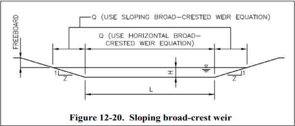
Figure 12-20. Sloping broad-crest weir
