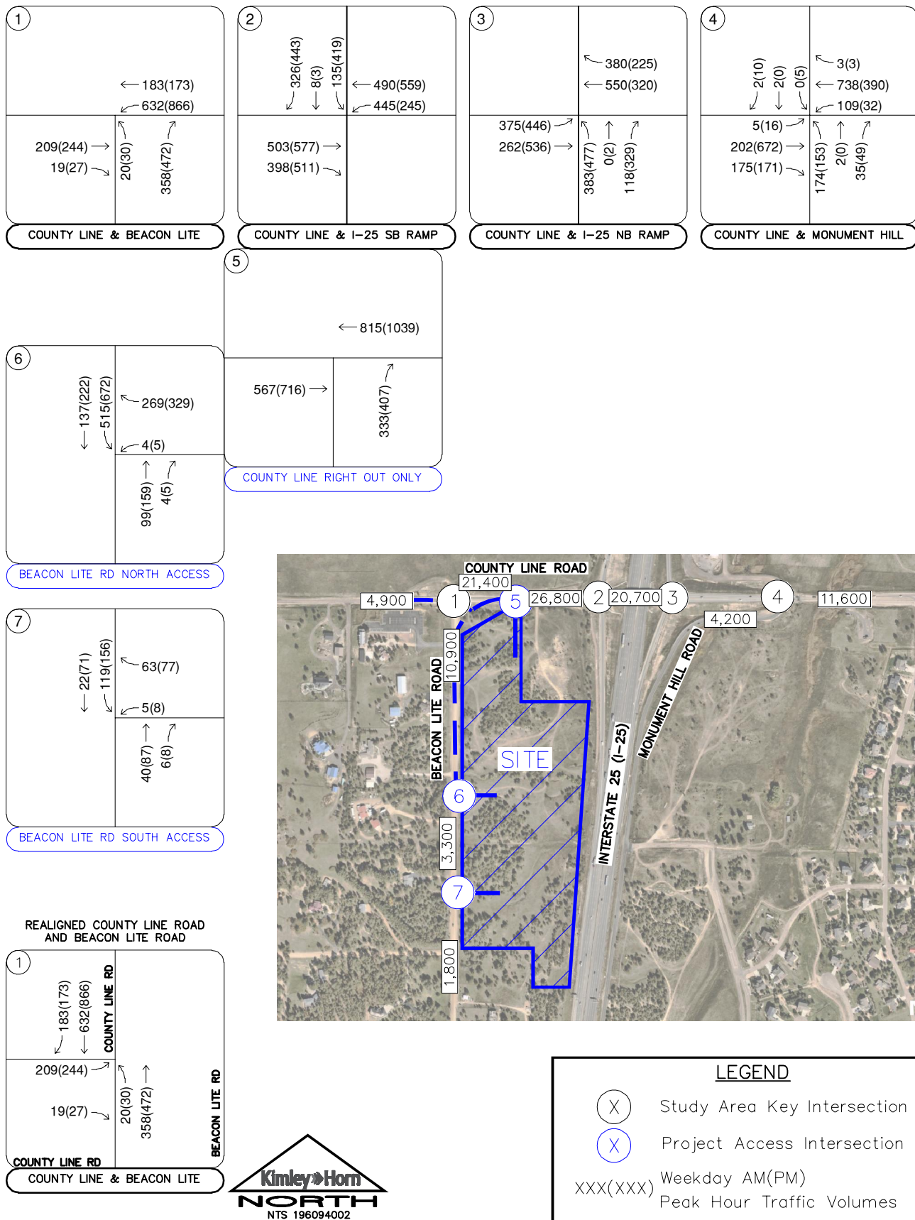
FIGURE 11 BUC-EE'S IH 25, EXIT 163 EL PASO COUNTY, COLORADO 2045 TOTAL TRAFFIC VOLUMES
