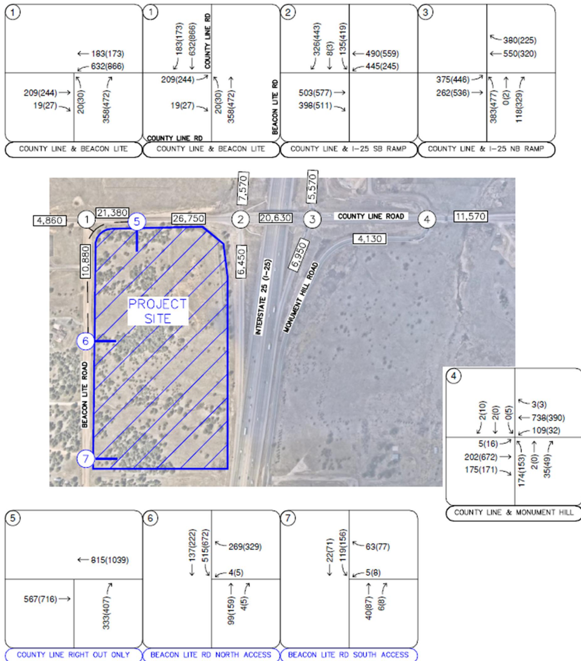
Figure 1 – 2045 Total Traffic Volumes
