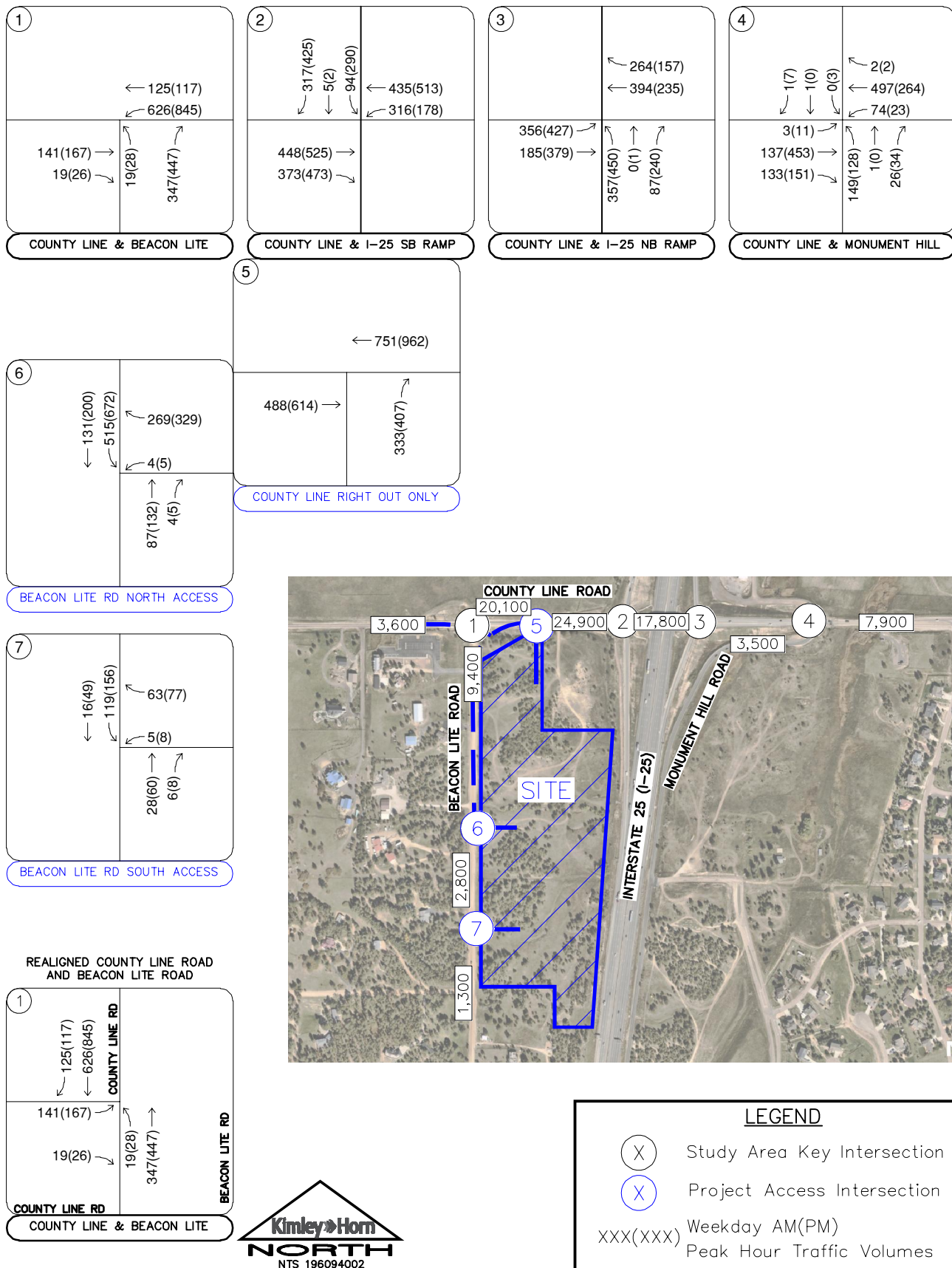
FIGURE 10 BUC-EE'S IH 25, EXIT 163 EL PASO COUNTY, COLORADO 2028 TOTAL TRAFFIC VOLUMES
