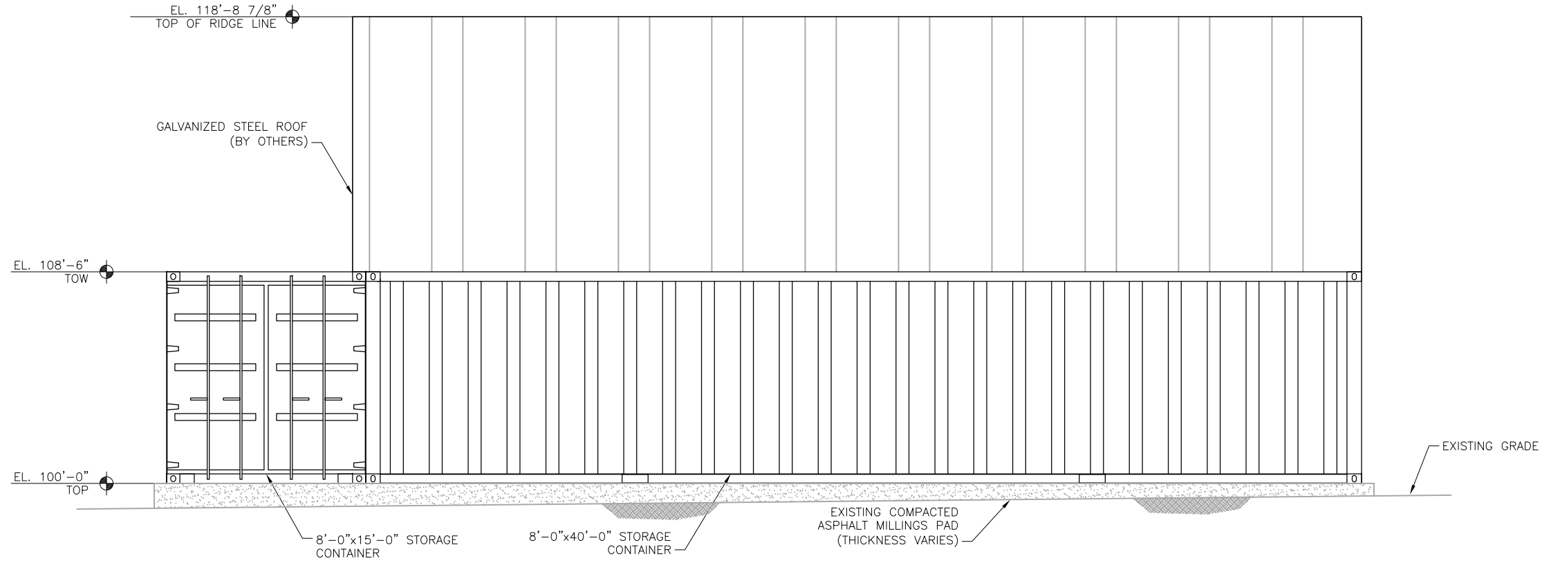
WEST ELEVATION SCALE: 3/16"=1'-0"
