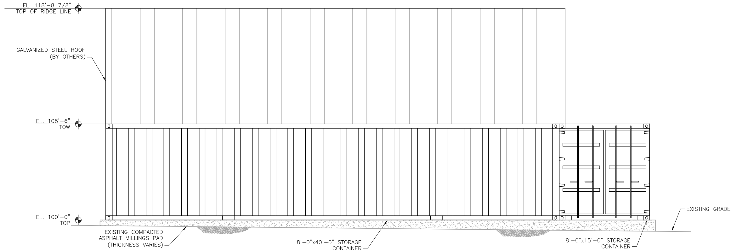
EAST ELEVATION SCALE: 3/16"=1'-0"
