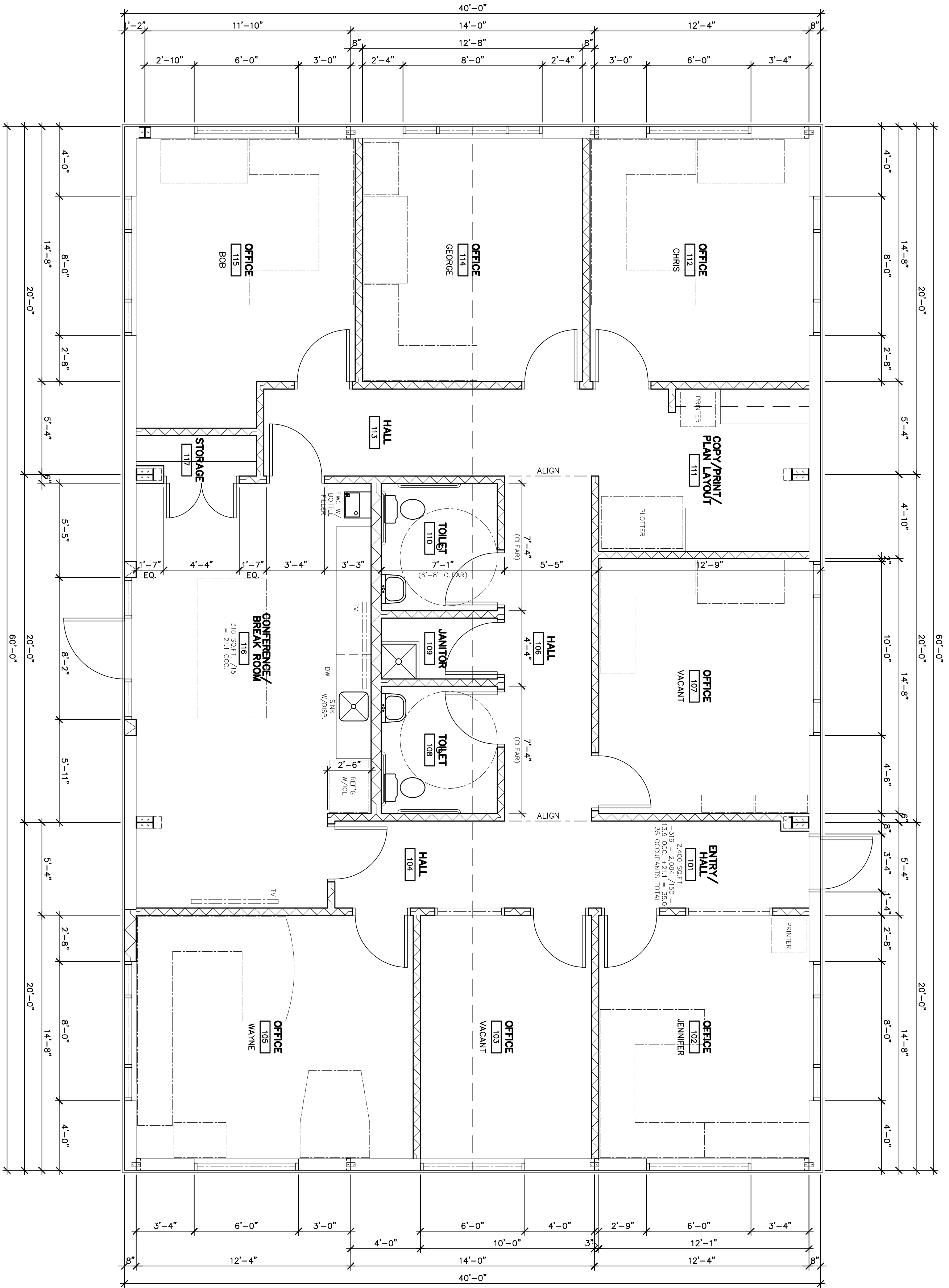
1 PROPOSED FLOOR PLAN 1/4" = 1'-0"
