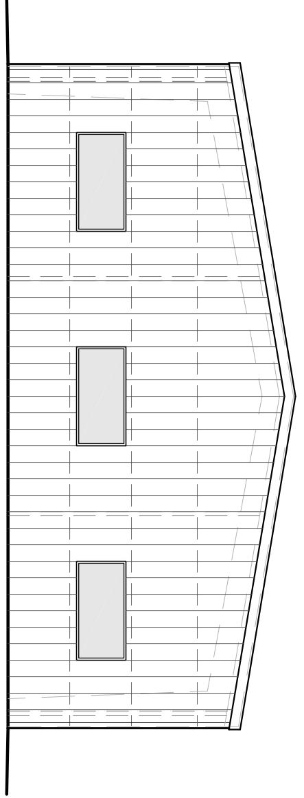
3 EAST ELEVATION 1/8" = 1'-0"
