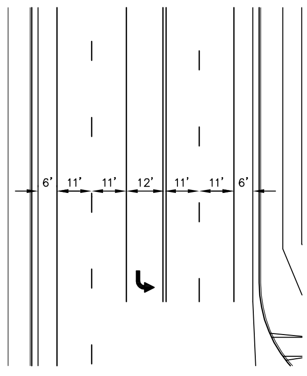
4-LANE MARKSHEFFEL ROAD STRIPING DETAIL SCALE: 1"=30' STA: 48+00 - 57+00
