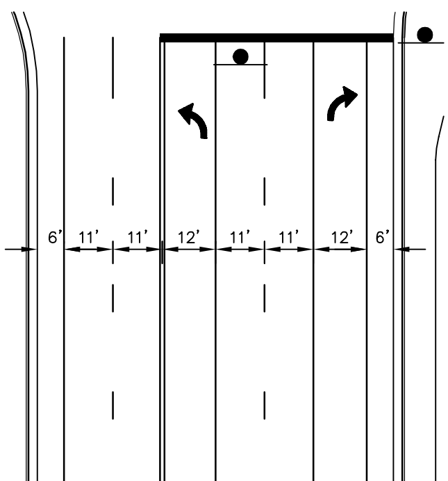
4-LANE MARKSHEFFEL ROAD STRIPING DETAIL SCALE: 1"=30' STA: 44+00 - 46+00
